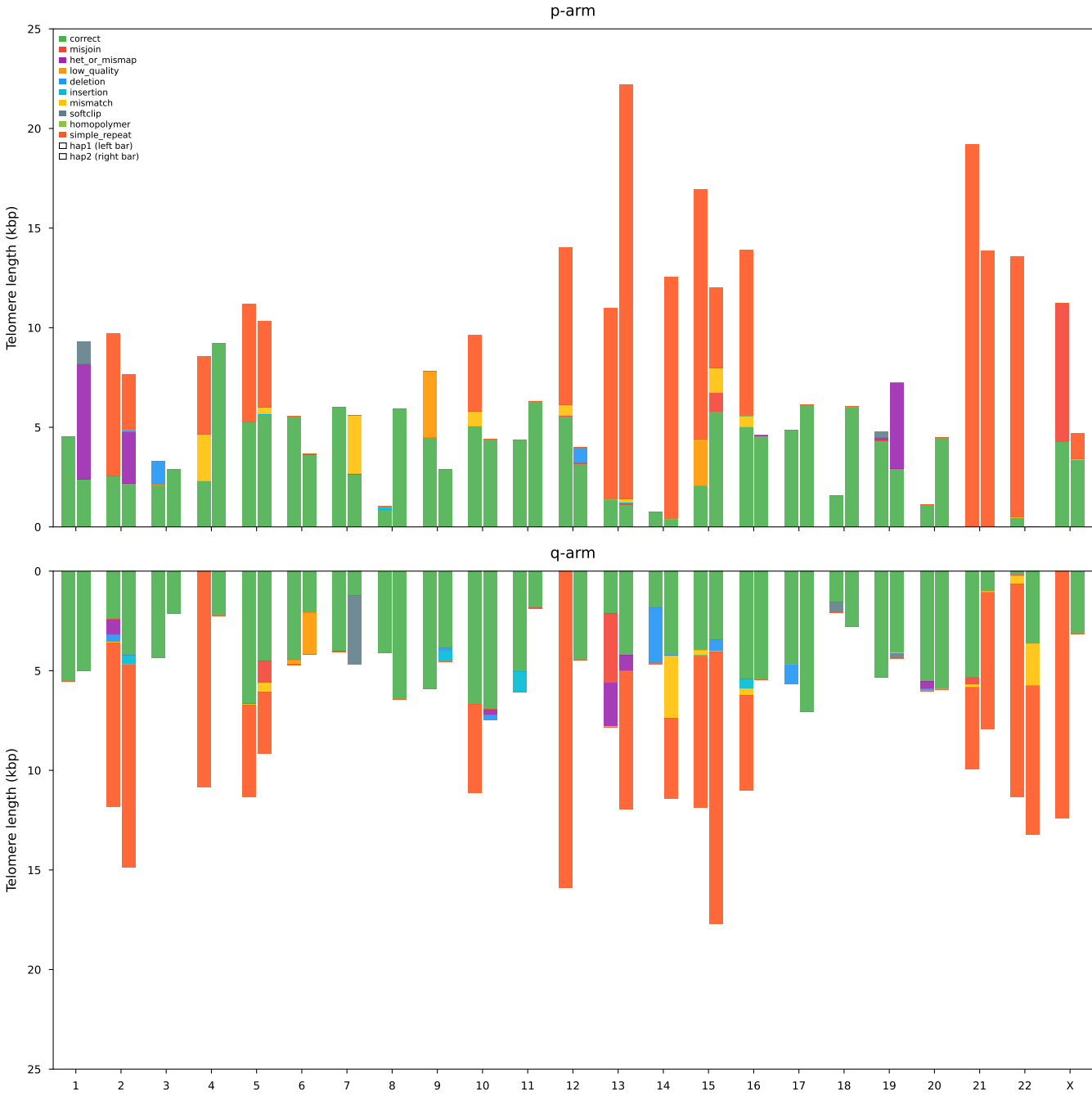
H9 telomere NucFlag annotation (HiFi)
