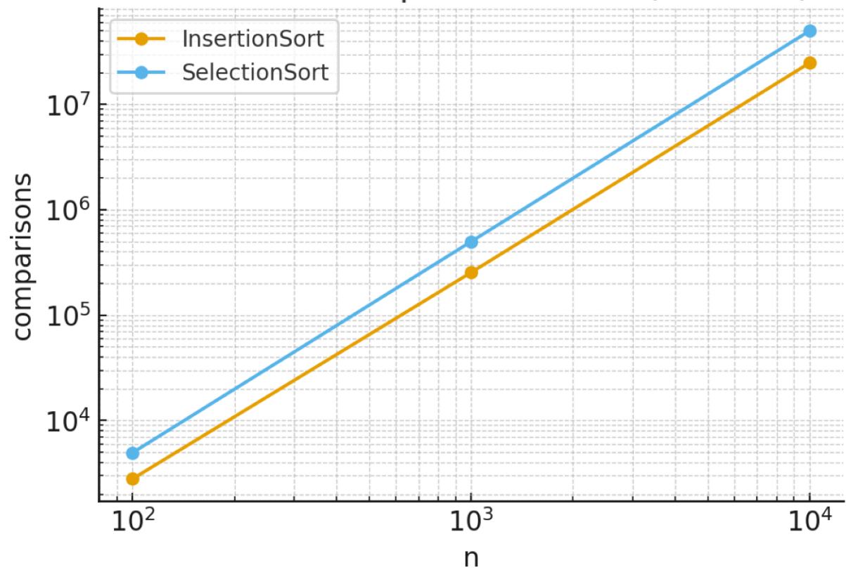
Real data: comparisons vs n (random)
