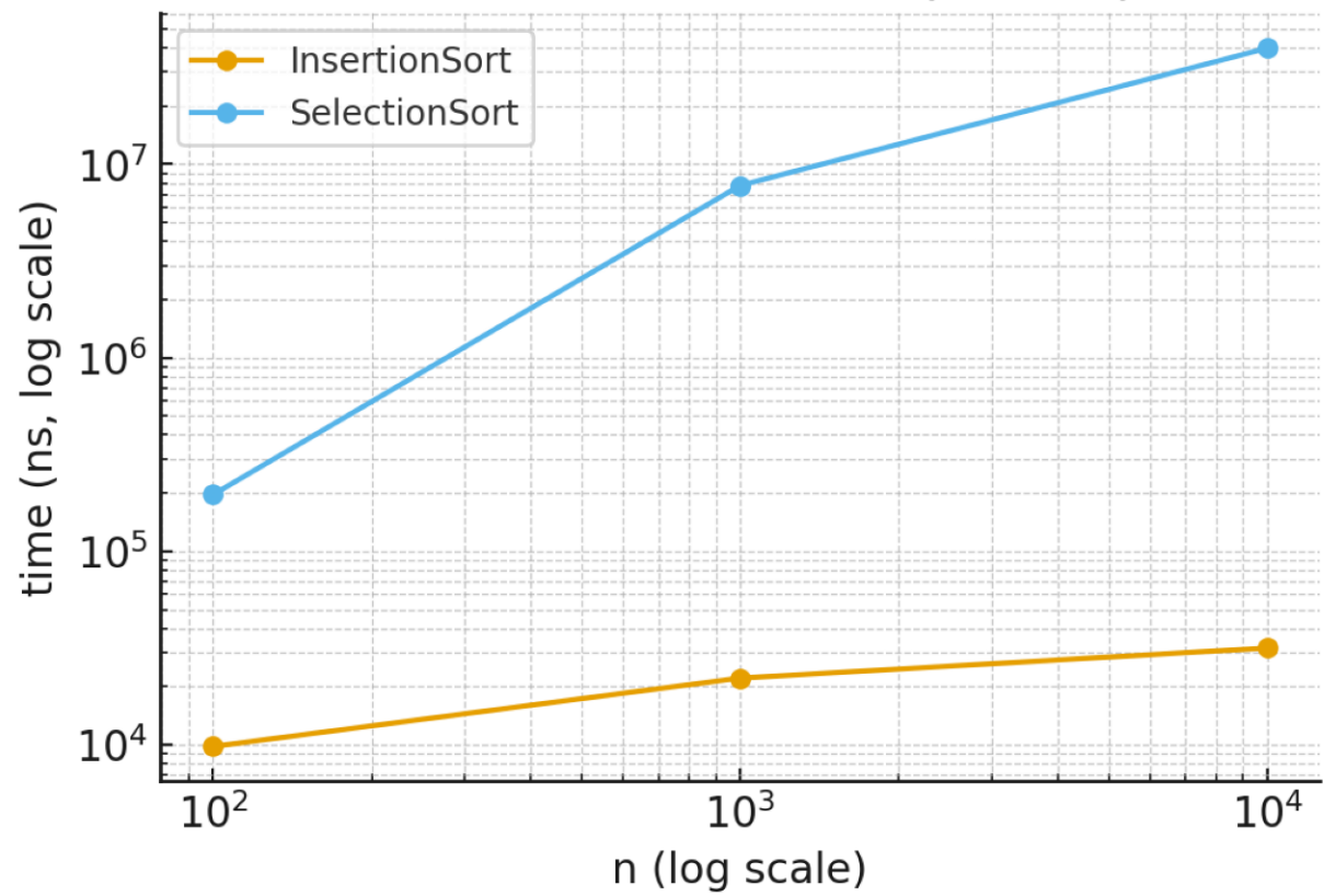
Real data: time vs n (sorted)
