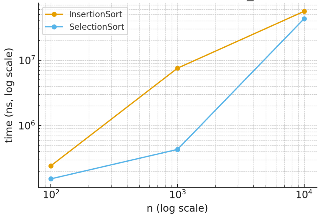
Real data: time vs n (reverse_sorted)
