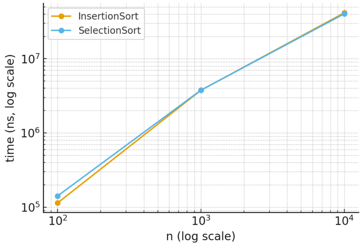
Real data: time vs n (random)
