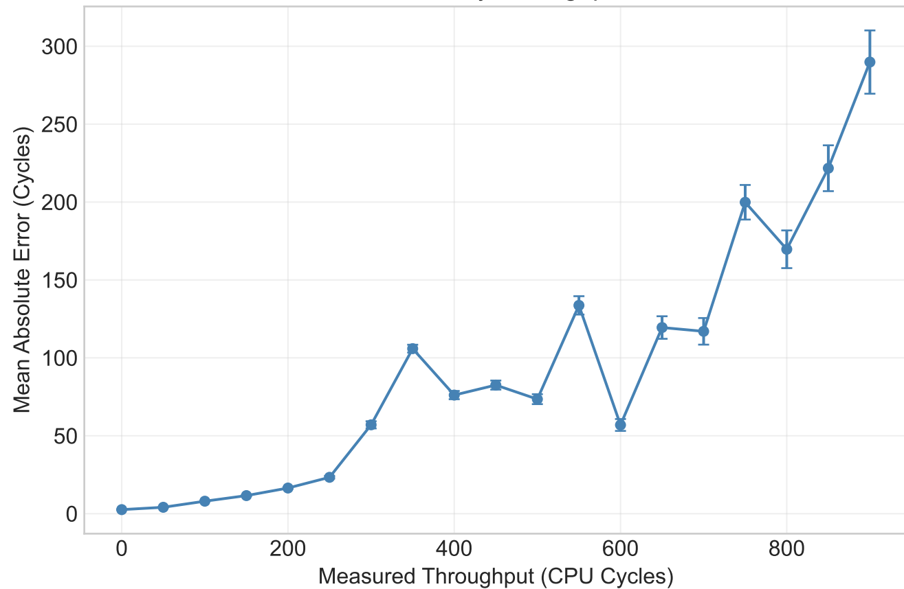
Absolute Error by Throughput - SKL
