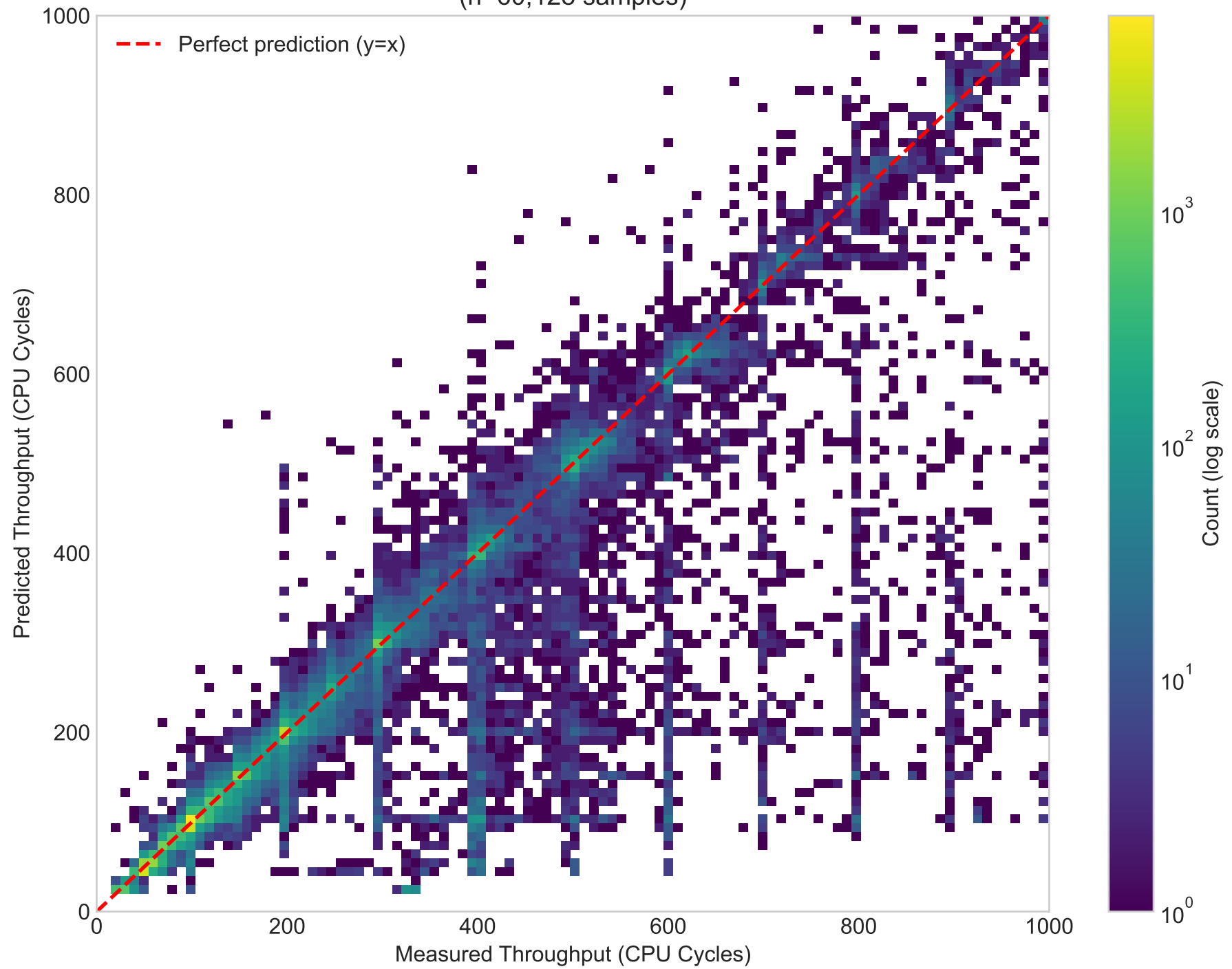
Ithermal Prediction Accuracy - SKL (n=60,128 samples)
