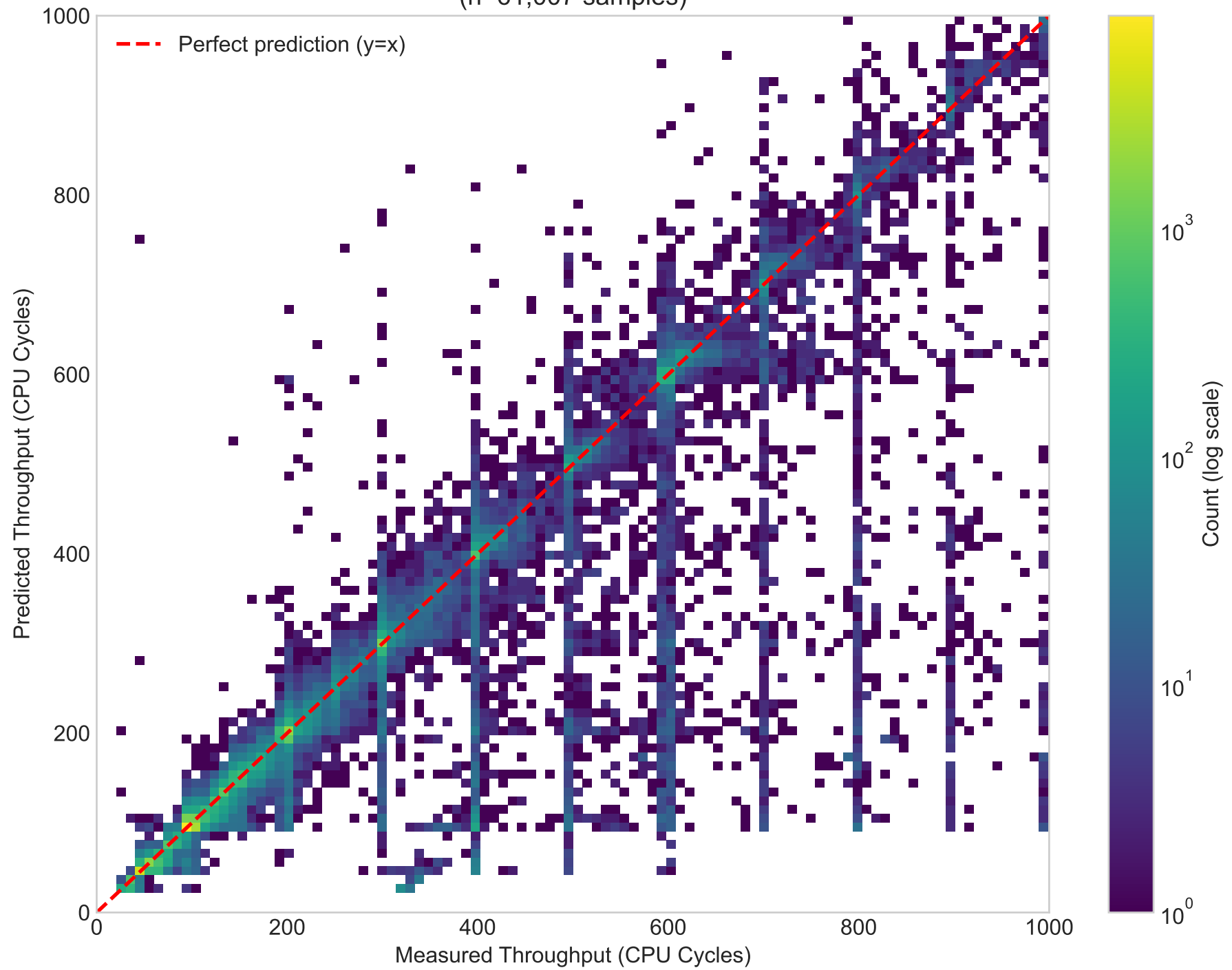
Ithema Prediction Accuracy - HSW (n=61,007 samples)
