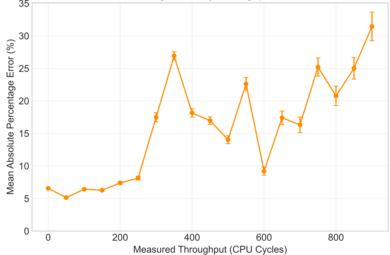
Percentage Error by Throughput - SKL
