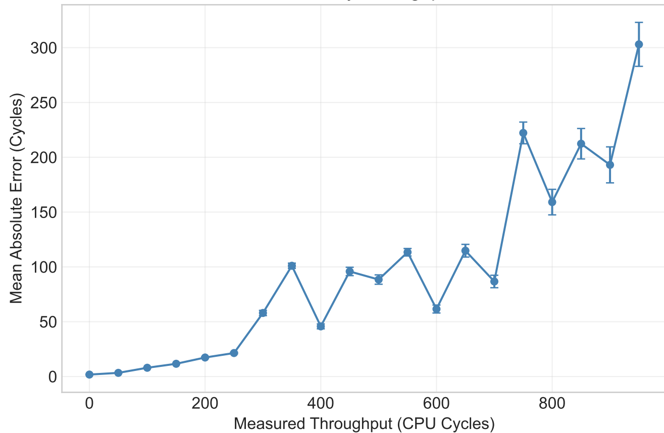
Absolute Error by Throughput - HSW
