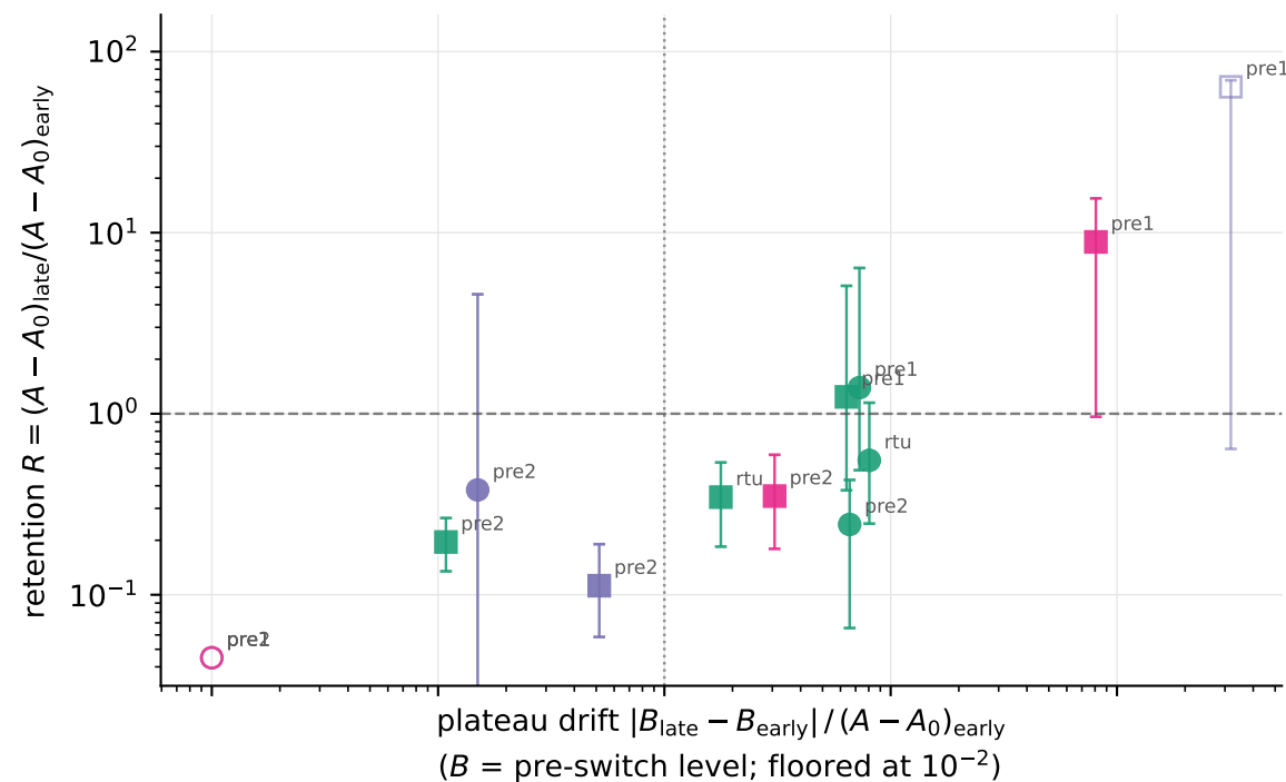
ActorCriticMLP
