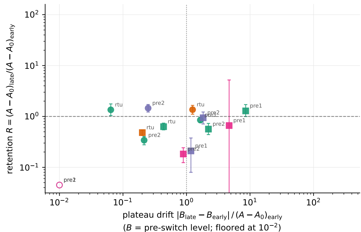
RealTimeActorCriticMLP
