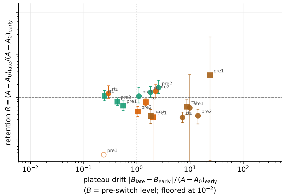
RealTimeActorCriticMLPReLU
