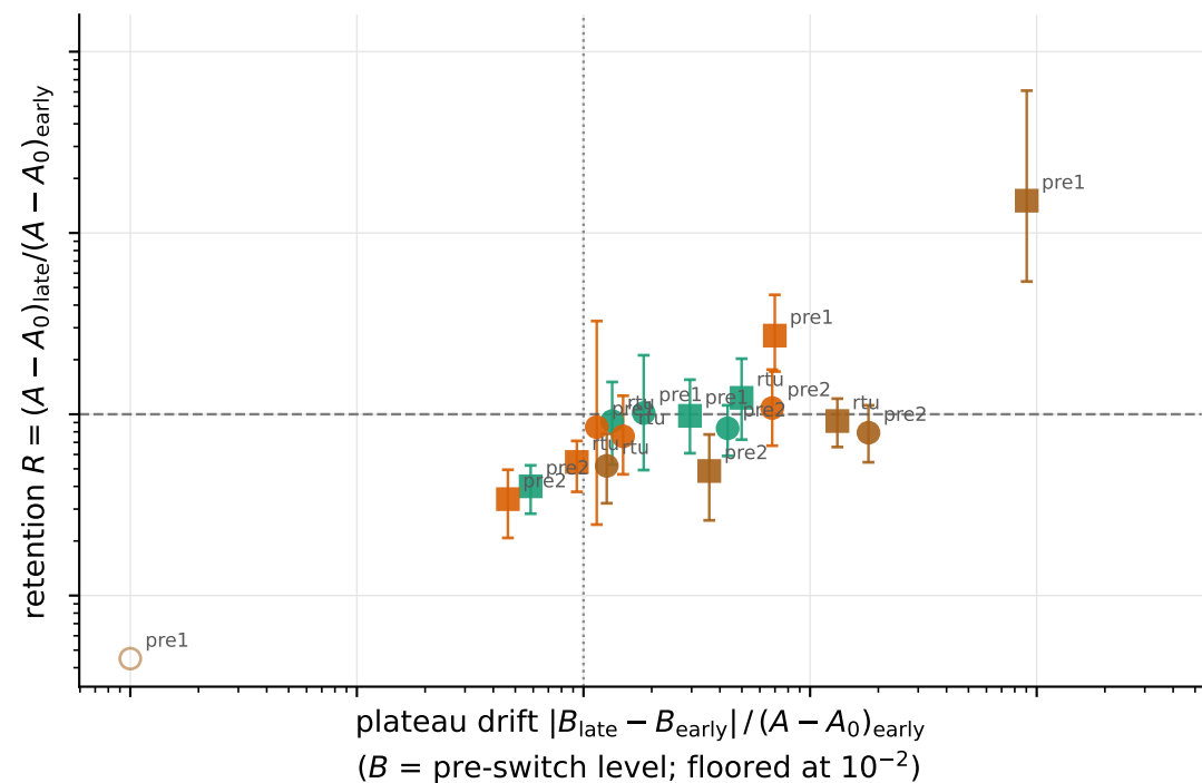
ActorCriticMLPReLU
