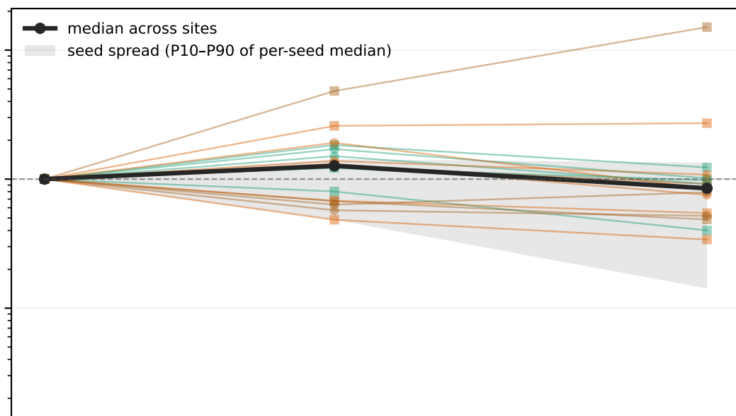
ActorCriticMLPReLU
