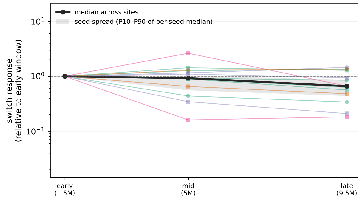
RealTimeActorCriticMLP
