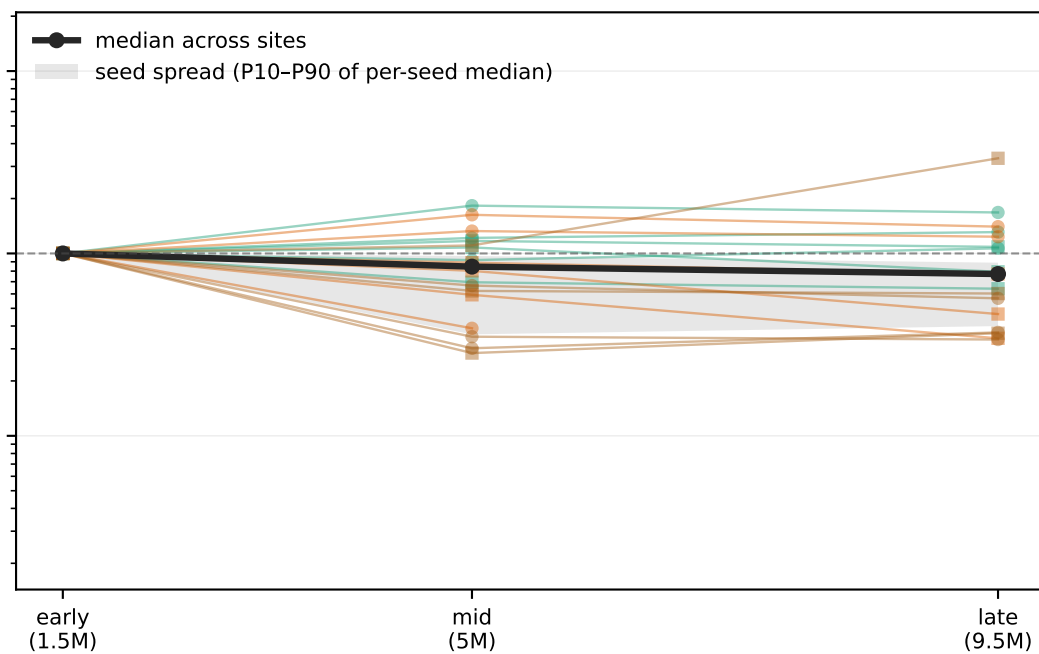
RealTimeActorCriticMLPReLU
