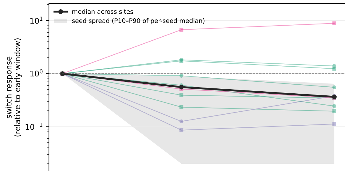
ActorCriticMLP
