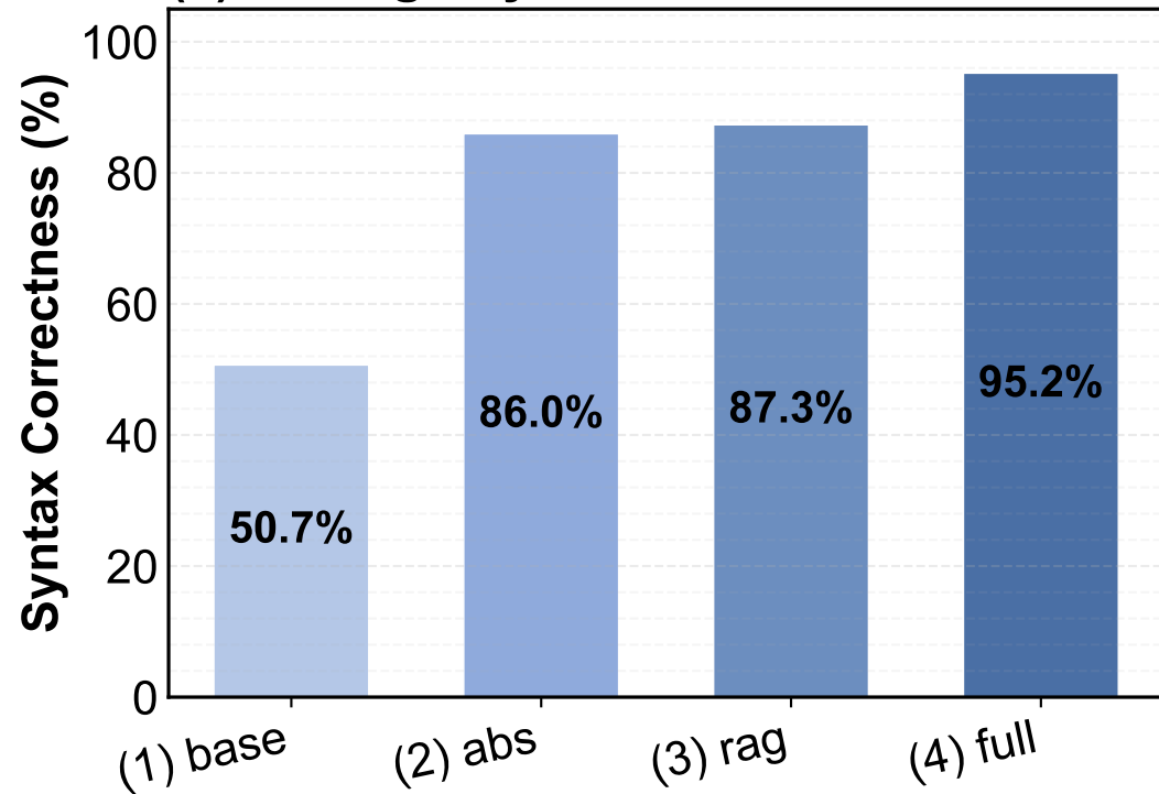
(a) Average Syntax Correctness Rate
