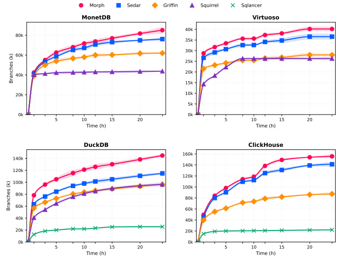
Fig. 7. Coverage growth over time in 24-hour fuzzing campaigns. Griffin denotes the downstream fuzzer with its original seed corpus.
