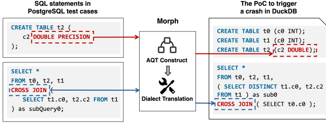
Fig. 6. An internal error found in DuckDB( Bug #205xx). Morph translates a test case of PostgreSQL to DuckDB while preserving critical data types and join logic.
