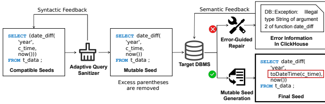
Fig. 5. Feedback-driven adaptive fuzzing workflow.
