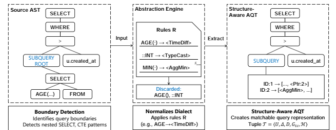
Fig. 3. An example of the per-statement component in AQT extraction. It detects nested SQL boundaries and normalizes dialect-specific features to abstract labels, producing the statement template used by the full test-case representation.
