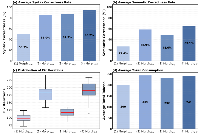
Fig. 8. Ablation analysis of Morph components.
