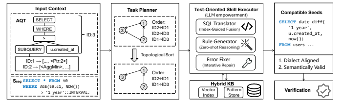
Fig. 4. RAG-enhanced AQT-Guided Dialect Instantiation.
