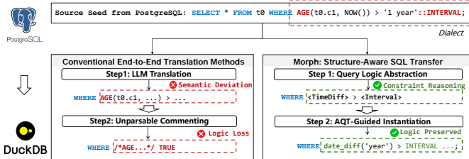
Fig. 1. Motivating example: Sedar causes semantic deviation and logic loss, while Morph preserves intent via AQT.
