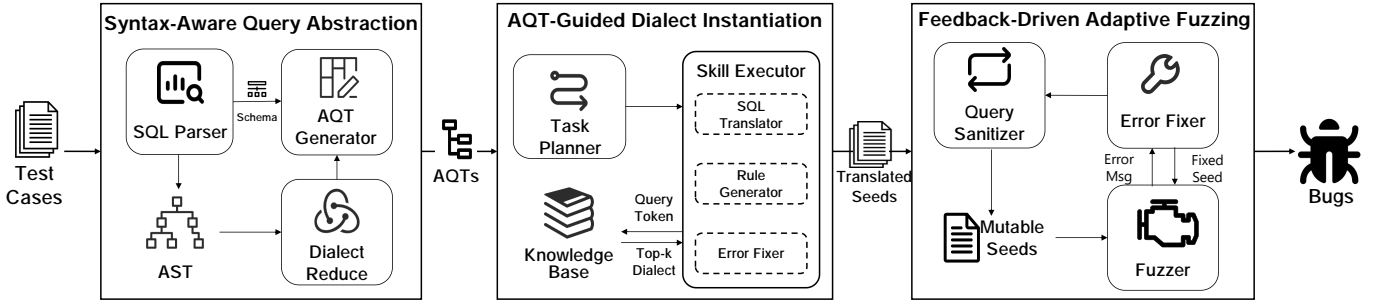
Fig. 2. Overview of Morph. Morph transfers source test cases through structure-preserving abstraction, AQT-Guided Dialect Instantiation, and feedback-driven adaptive fuzzing.
