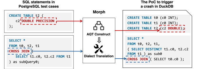
Fig. 6. An internal error found in DuckDB( Bug #205xx). MORPH translates a test case of PostgreSQL to DuckDB while preserving critical data types and join logic.
