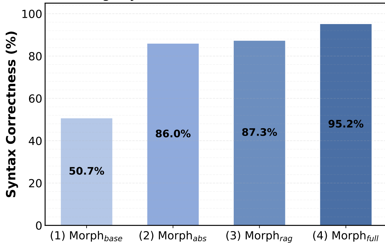
(a) Average Syntax Correctness Rate
