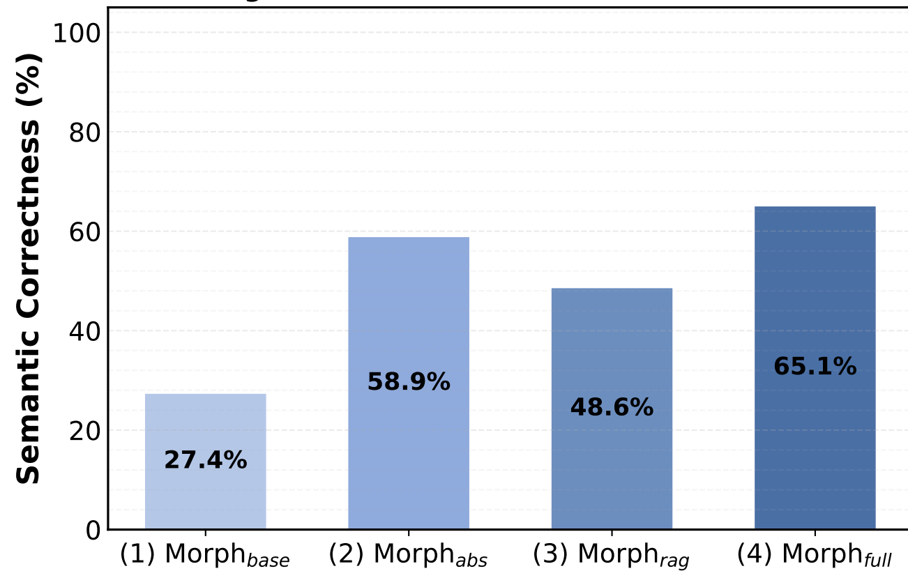
(b) Average Semantic Correctness Rate
