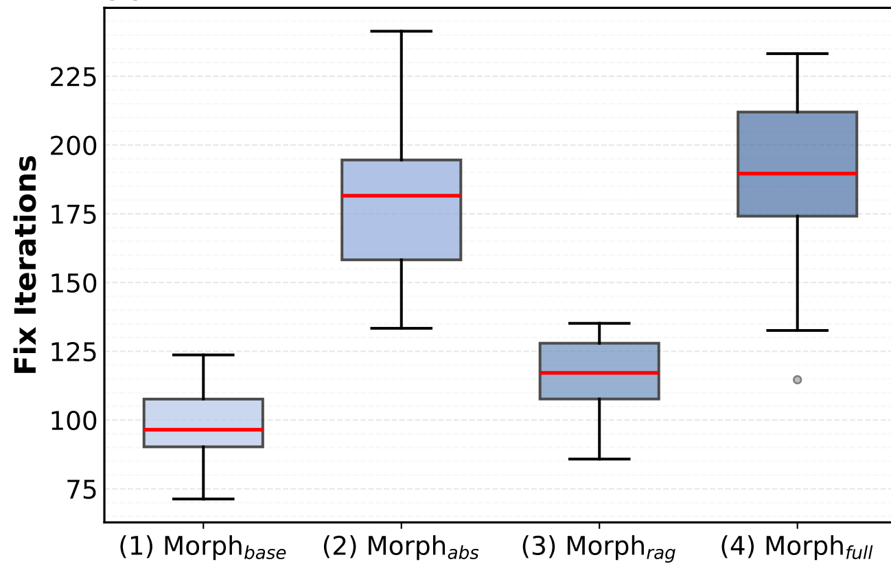
(c) Distribution of Fix Iterations
