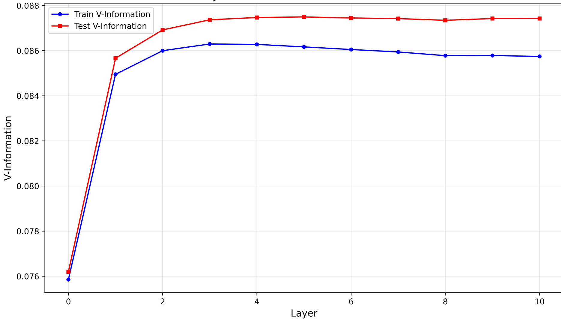
Layer-wise V-Information on Diabetes
