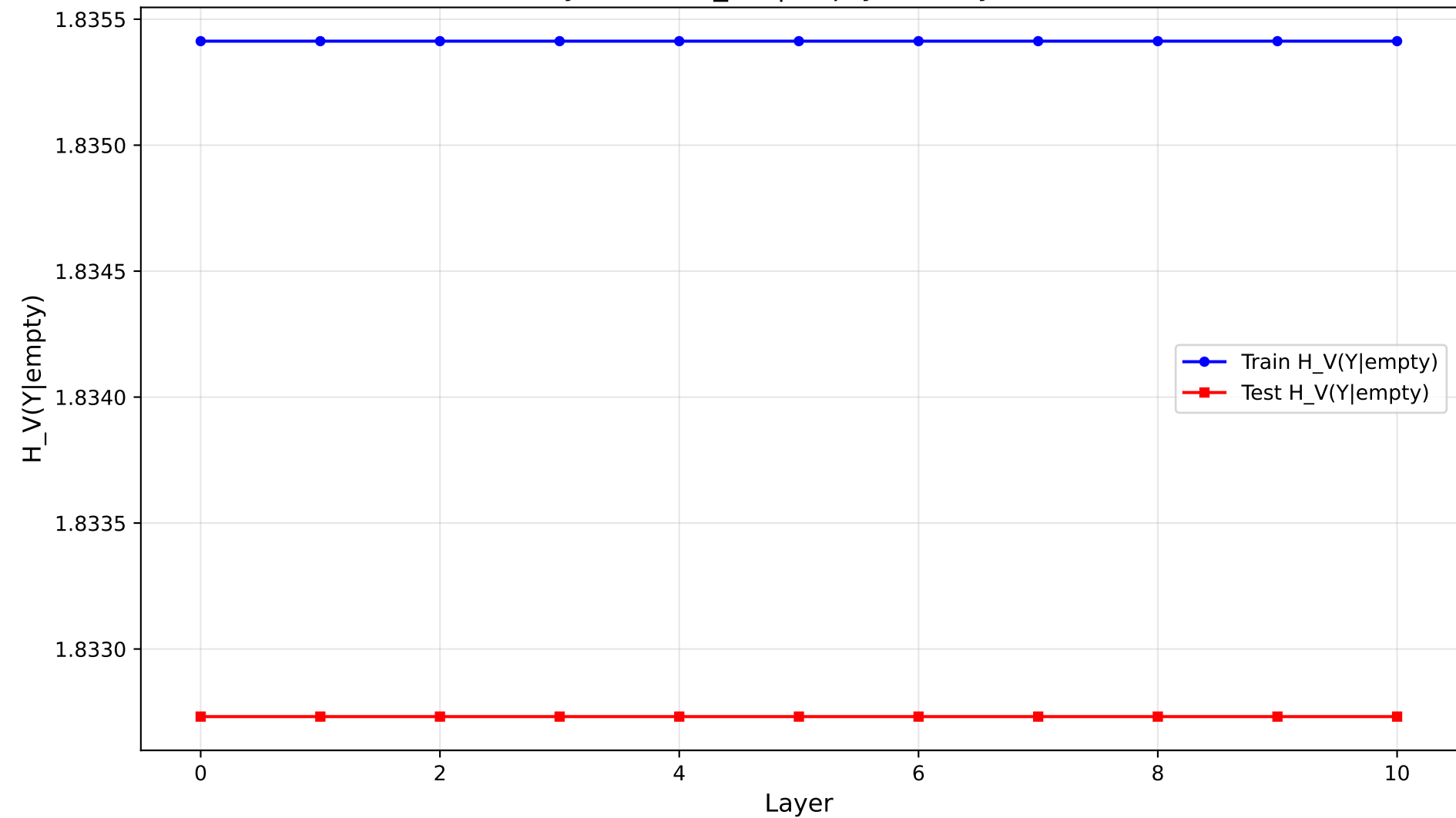
Layer-wise H_V(Y|\text{empty}) on DryBean
