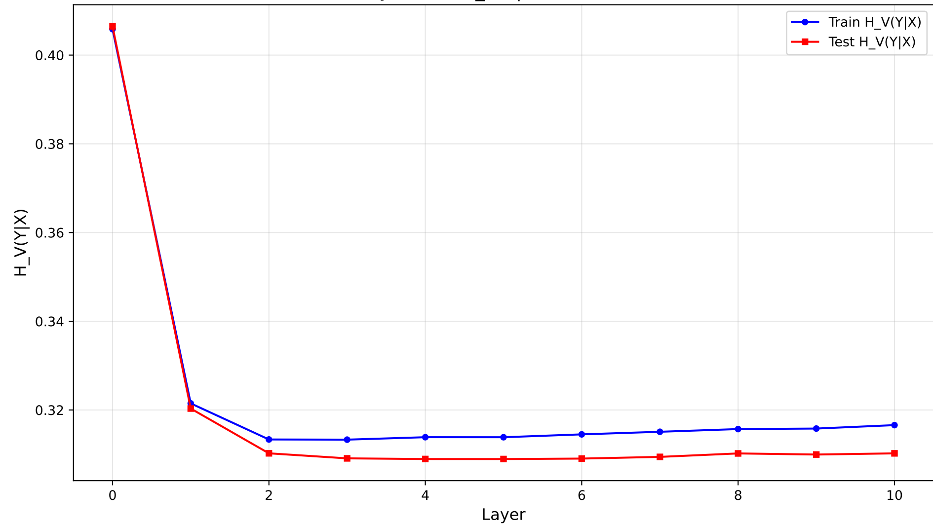
Layer-wise H_V(Y|X) on Gamma
