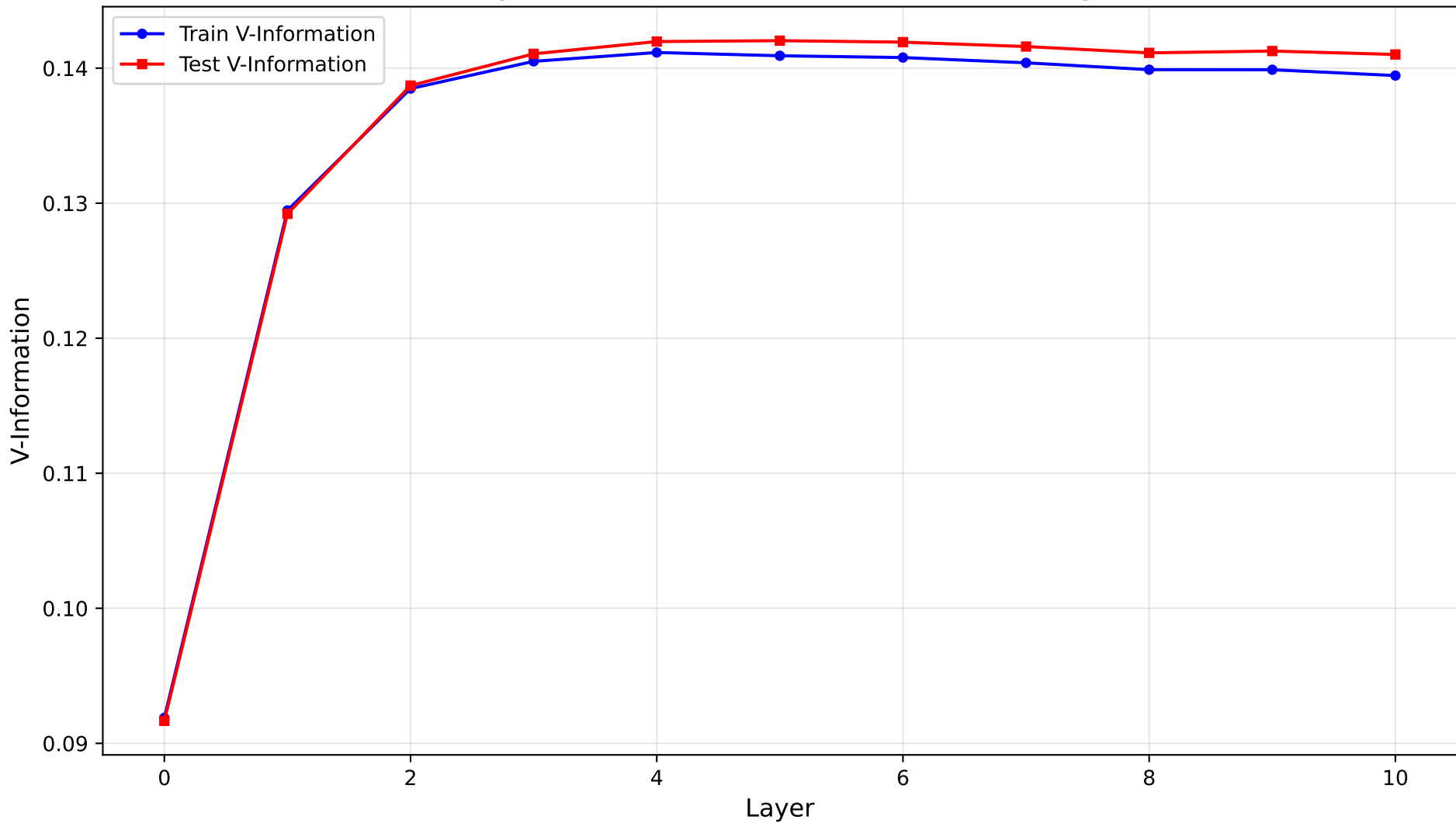
Layer-wise V-Information on BankMarketing
