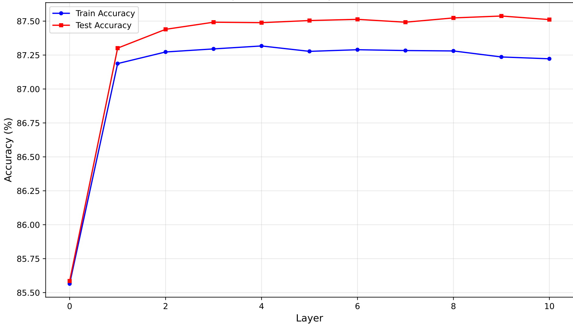
Layer-wise Accuracy on Gamma
