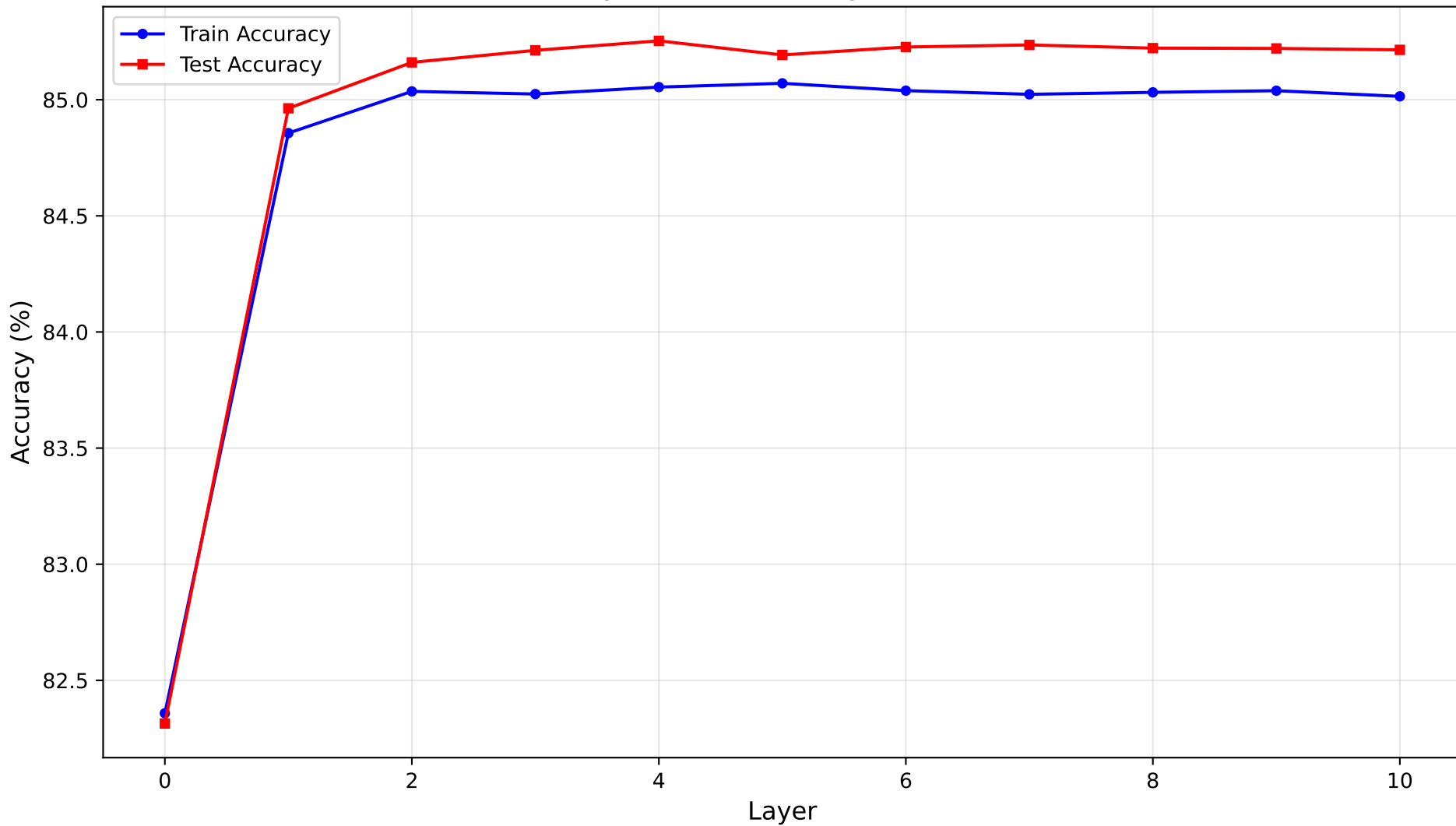
Layer-wise Accuracy on Adult
