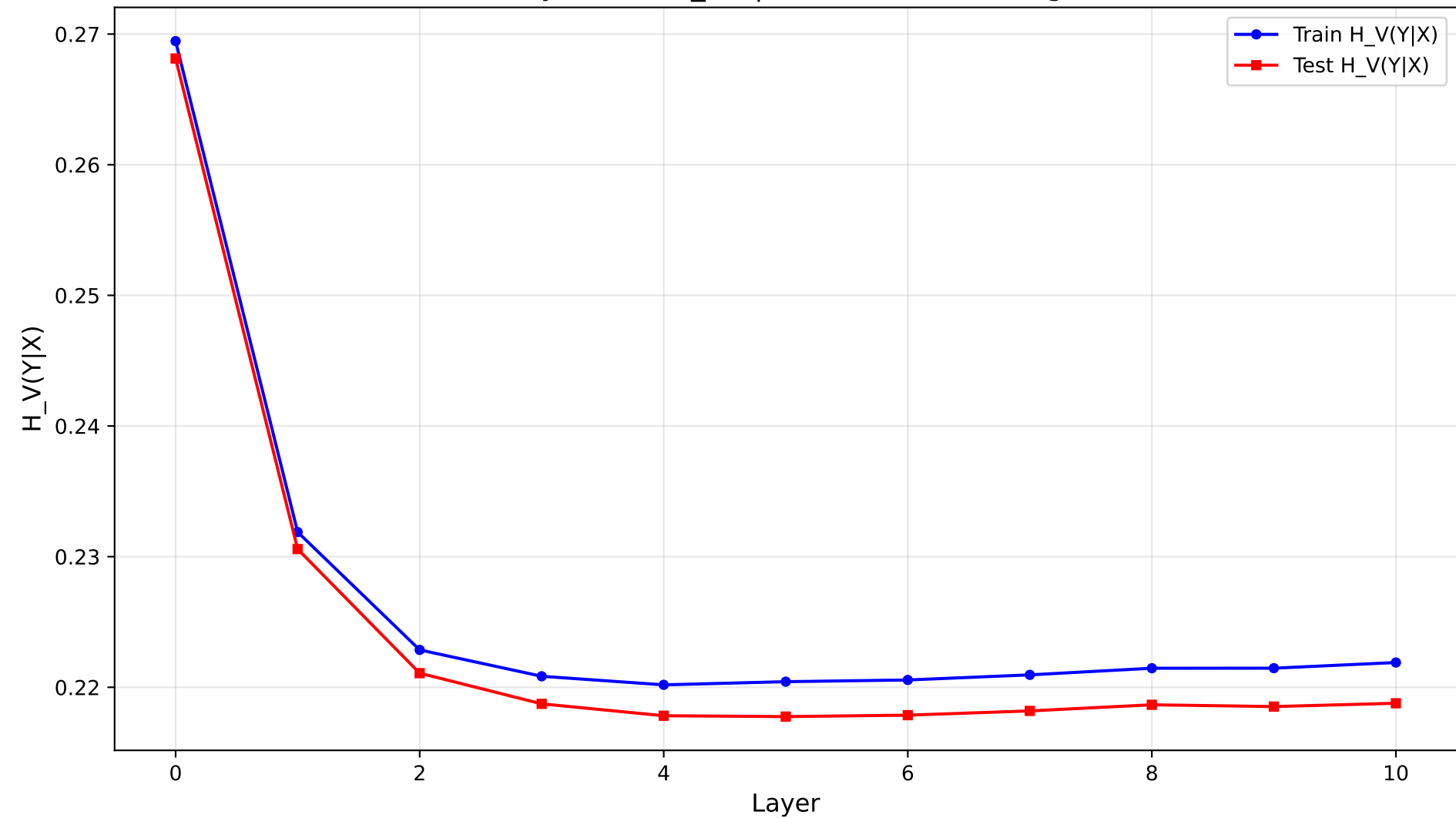
Layer-wise H_V(Y|X) on BankMarketing
