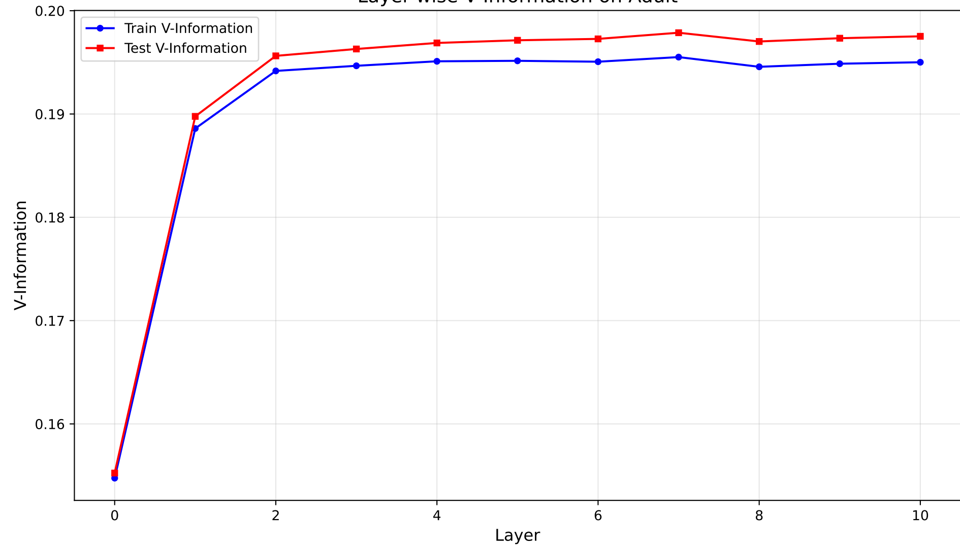
Layer-wise V-Information on Adult
