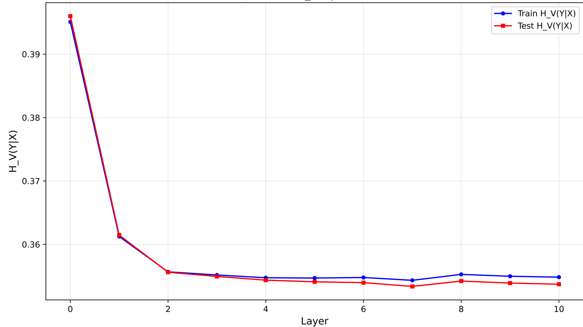
Layer-wise H_V(Y|X) on Adult
