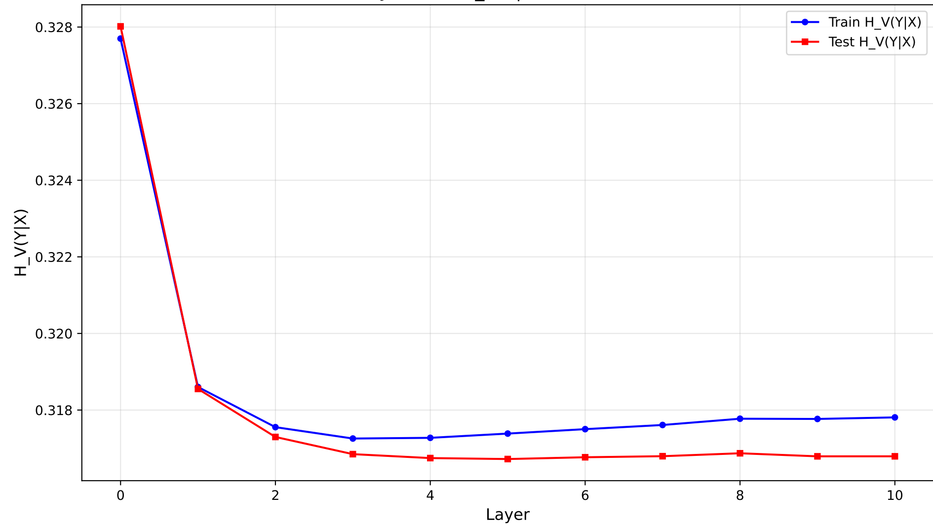
Layer-wise H_V(Y|X) on Diabetes
