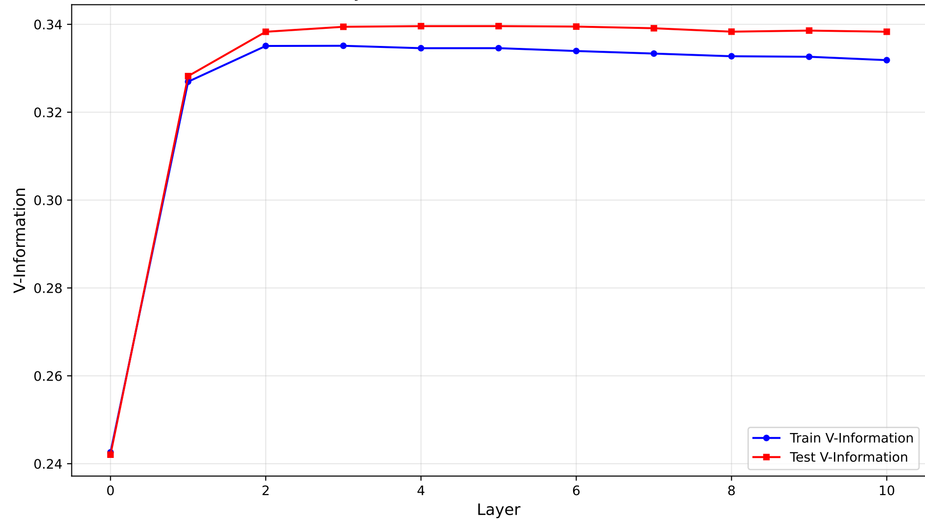
Layer-wise V-Information on Gamma
