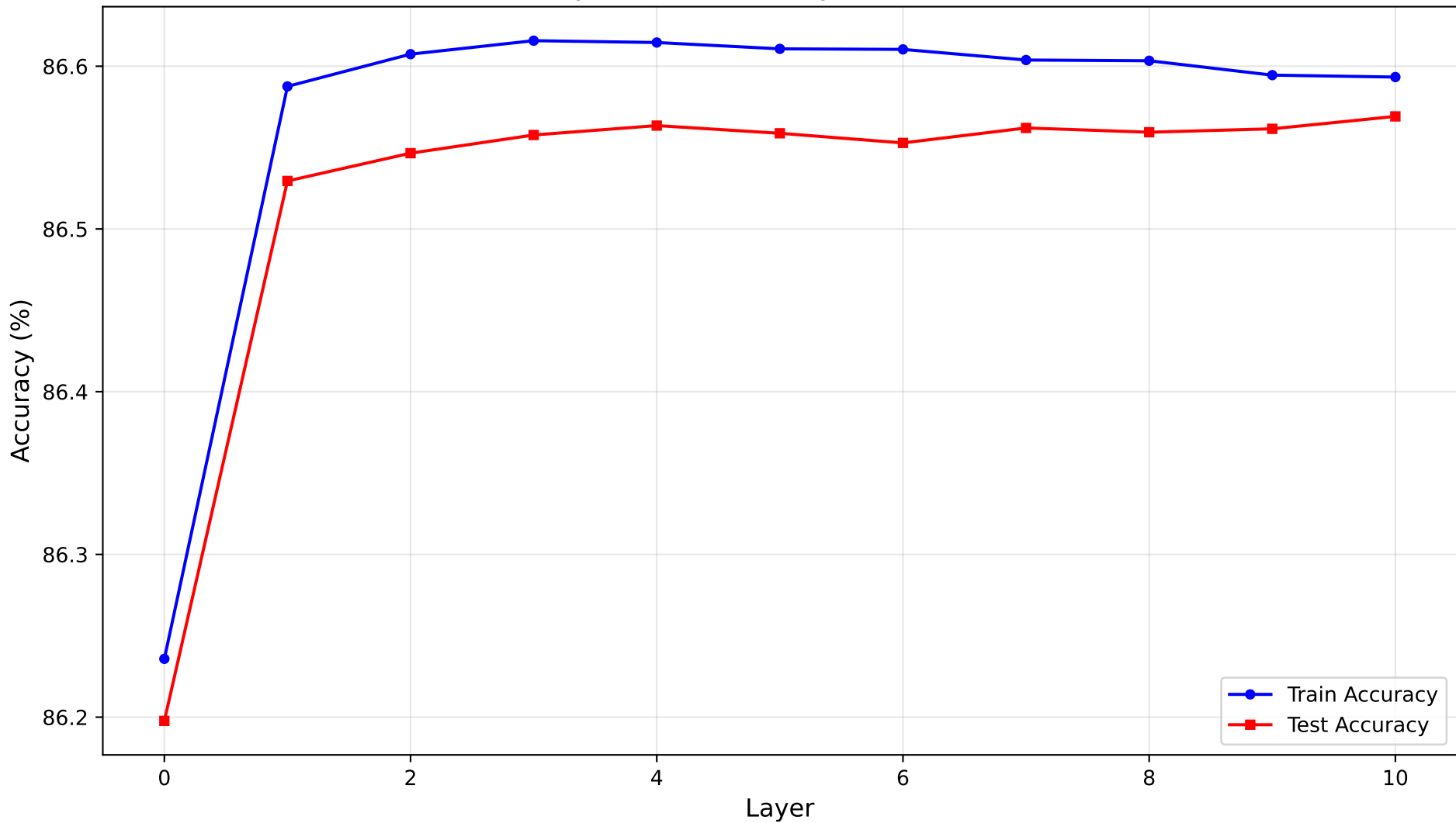
Layer-wise Accuracy on Diabetes
