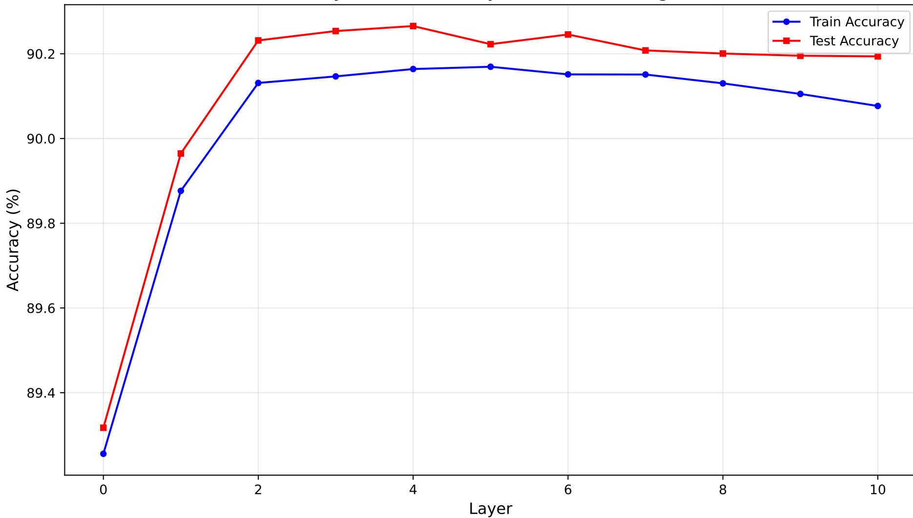
Layer-wise Accuracy on BankMarketing
