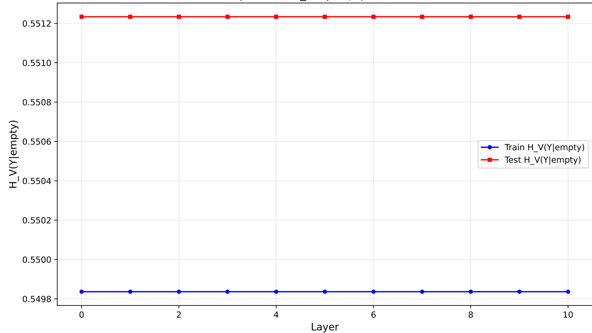
Layer-wise H_V(Y|\text{empty}) on Adult
