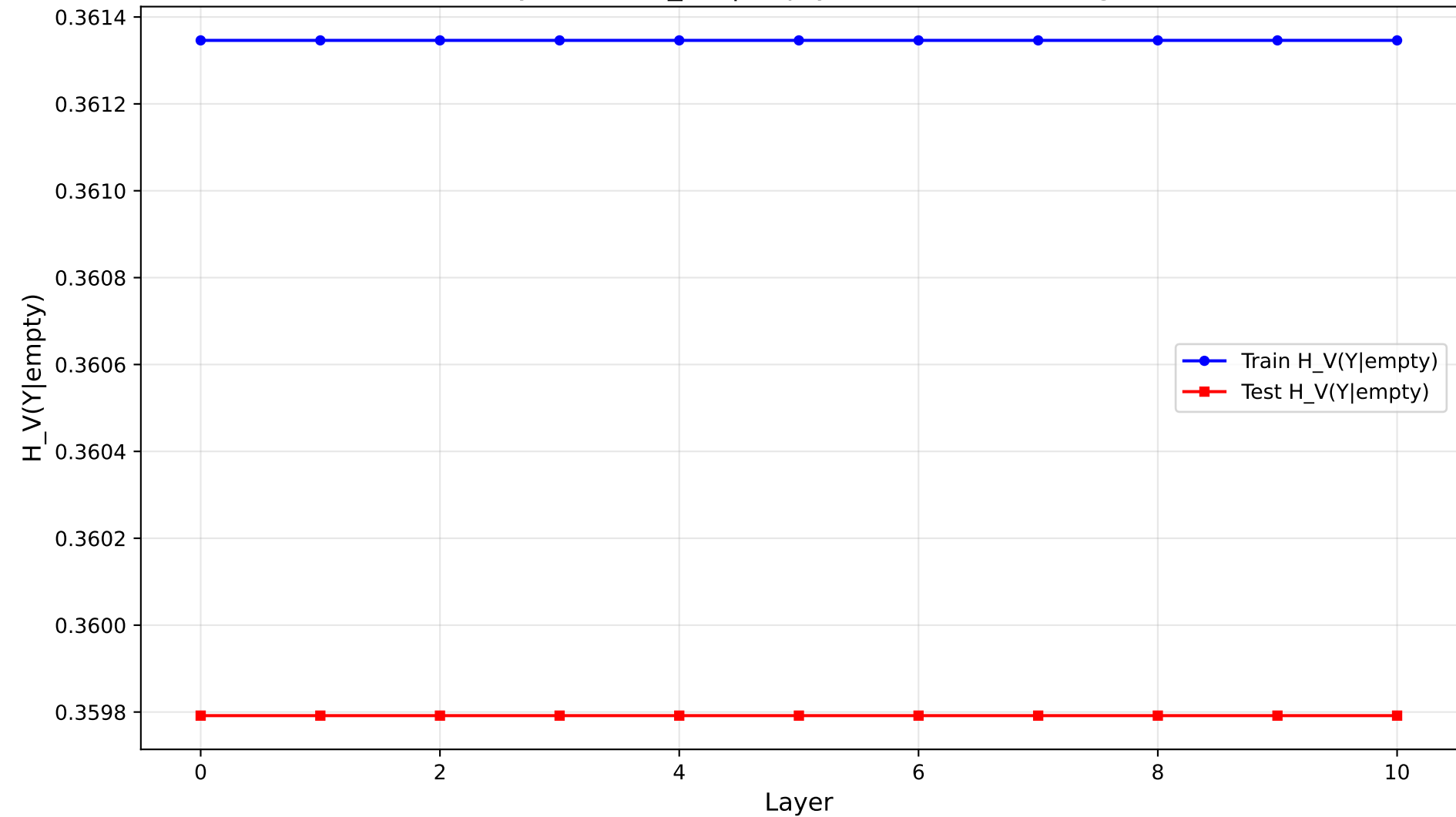
Layer-wise H_V(Y|\text{empty}) on BankMarketing
