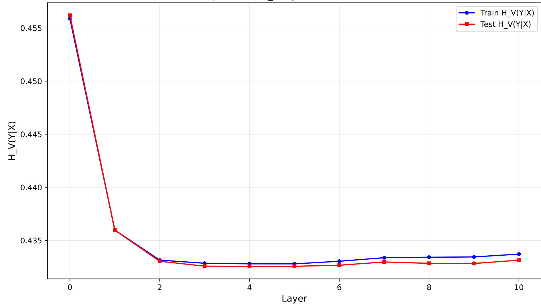
Layer-wise H_V(Y|X) on CreditCard
