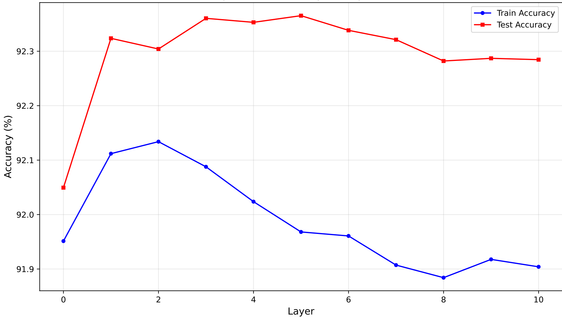
Layer-wise Accuracy on DryBean
