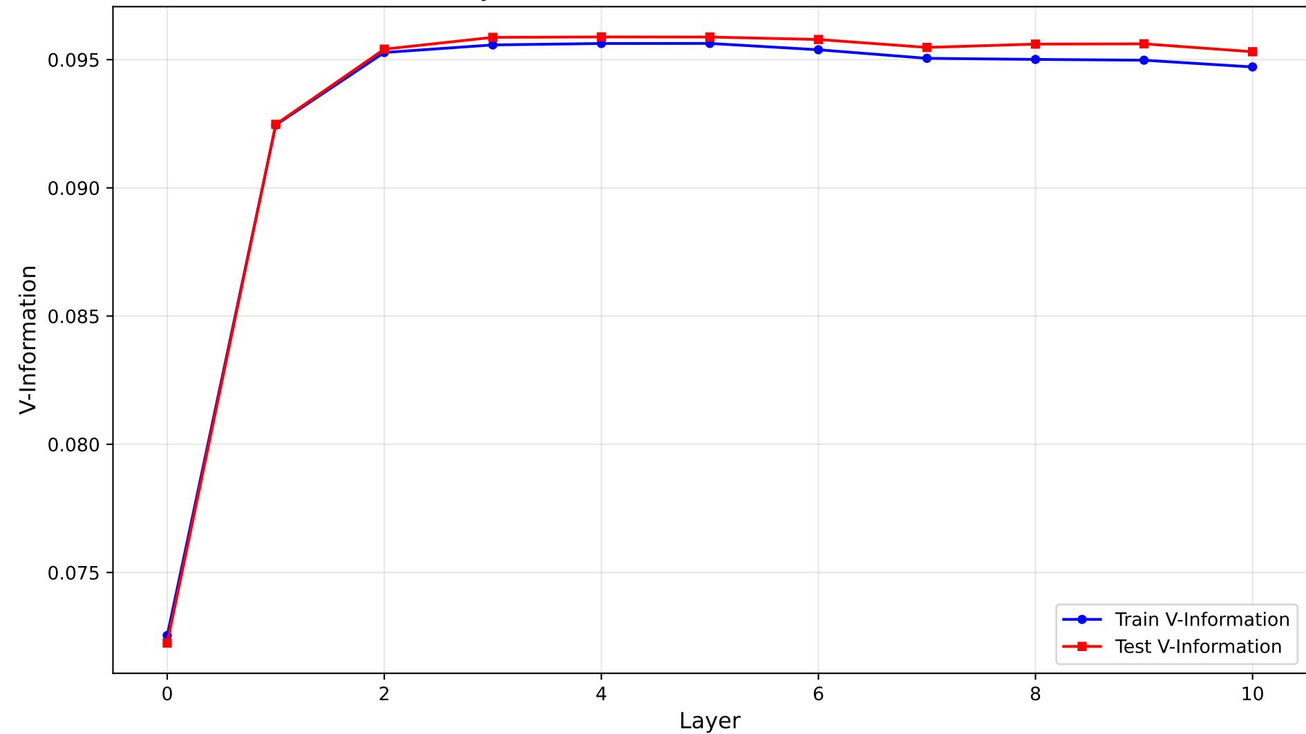
Layer-wise V-Information on CreditCard
