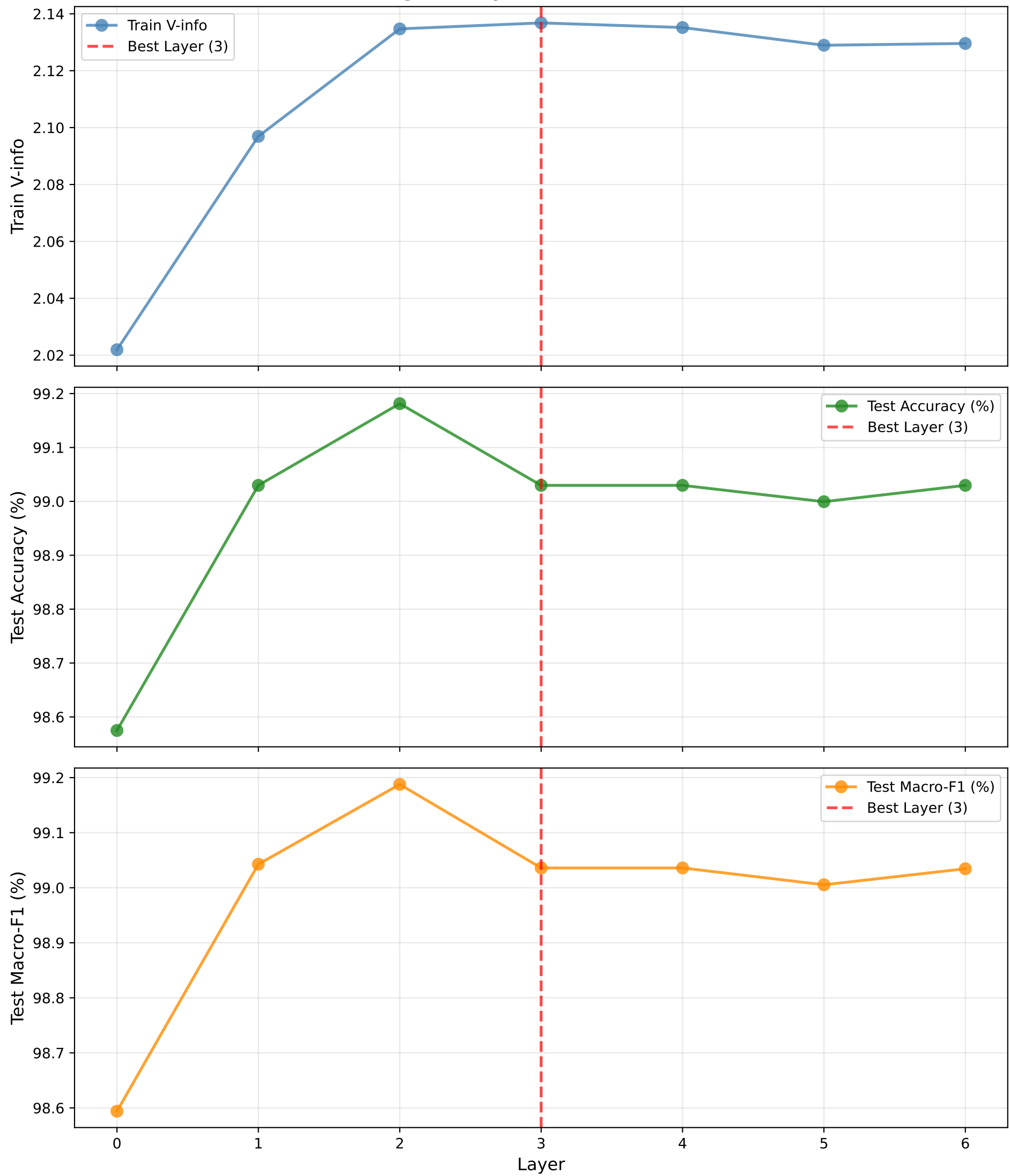
Pendigits - Layer-wise Metrics
