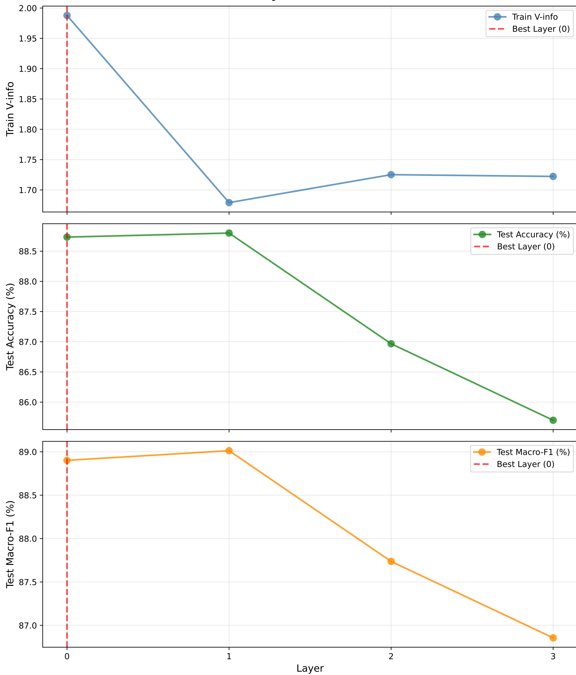
Letter - Layer-wise Metrics
