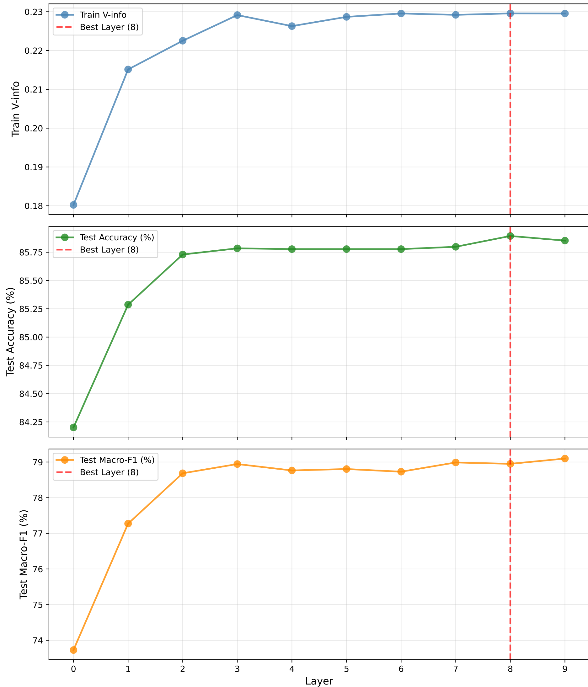
Adult - Layer-wise Metrics
