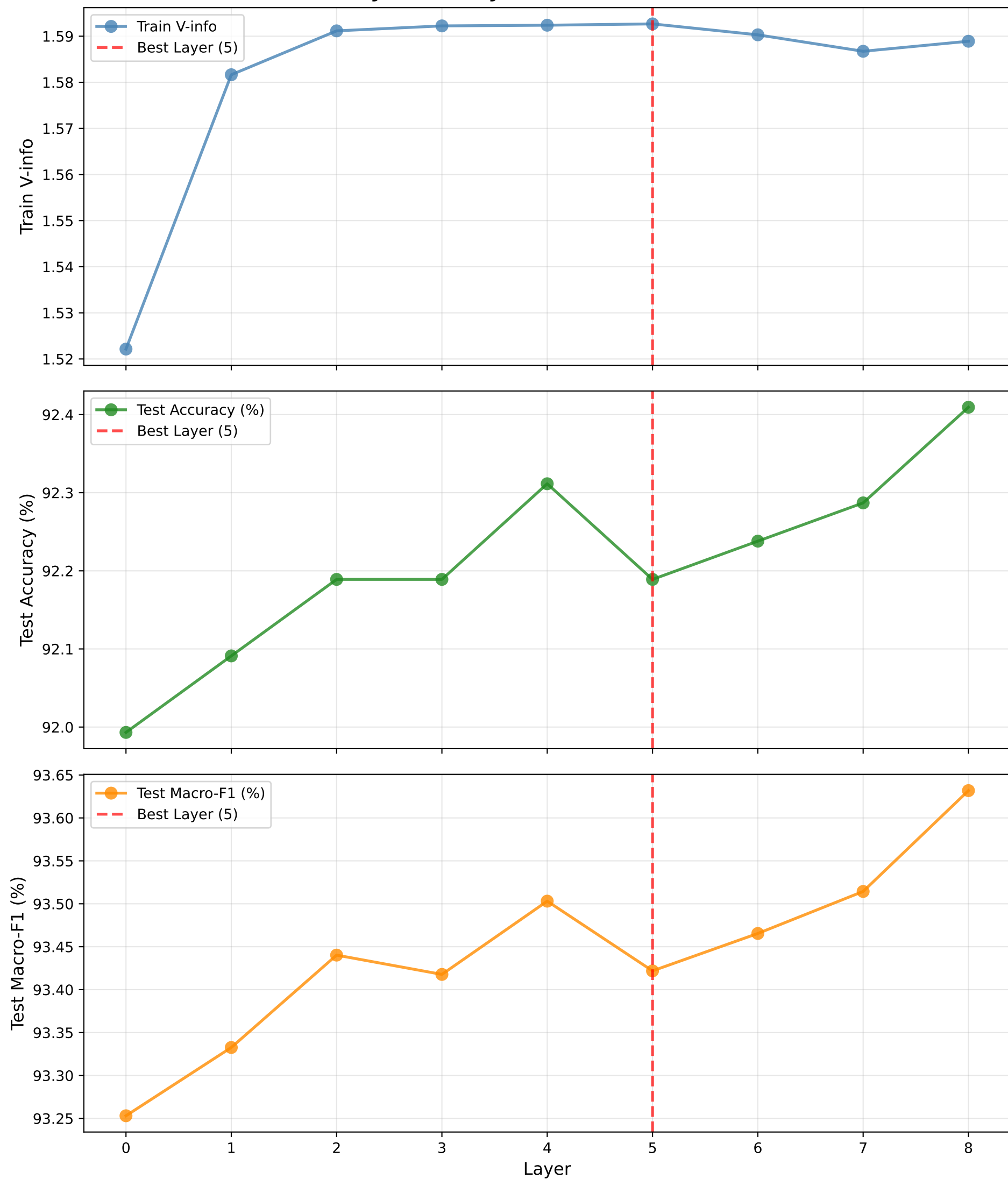
DryBean - Layer-wise Metrics
