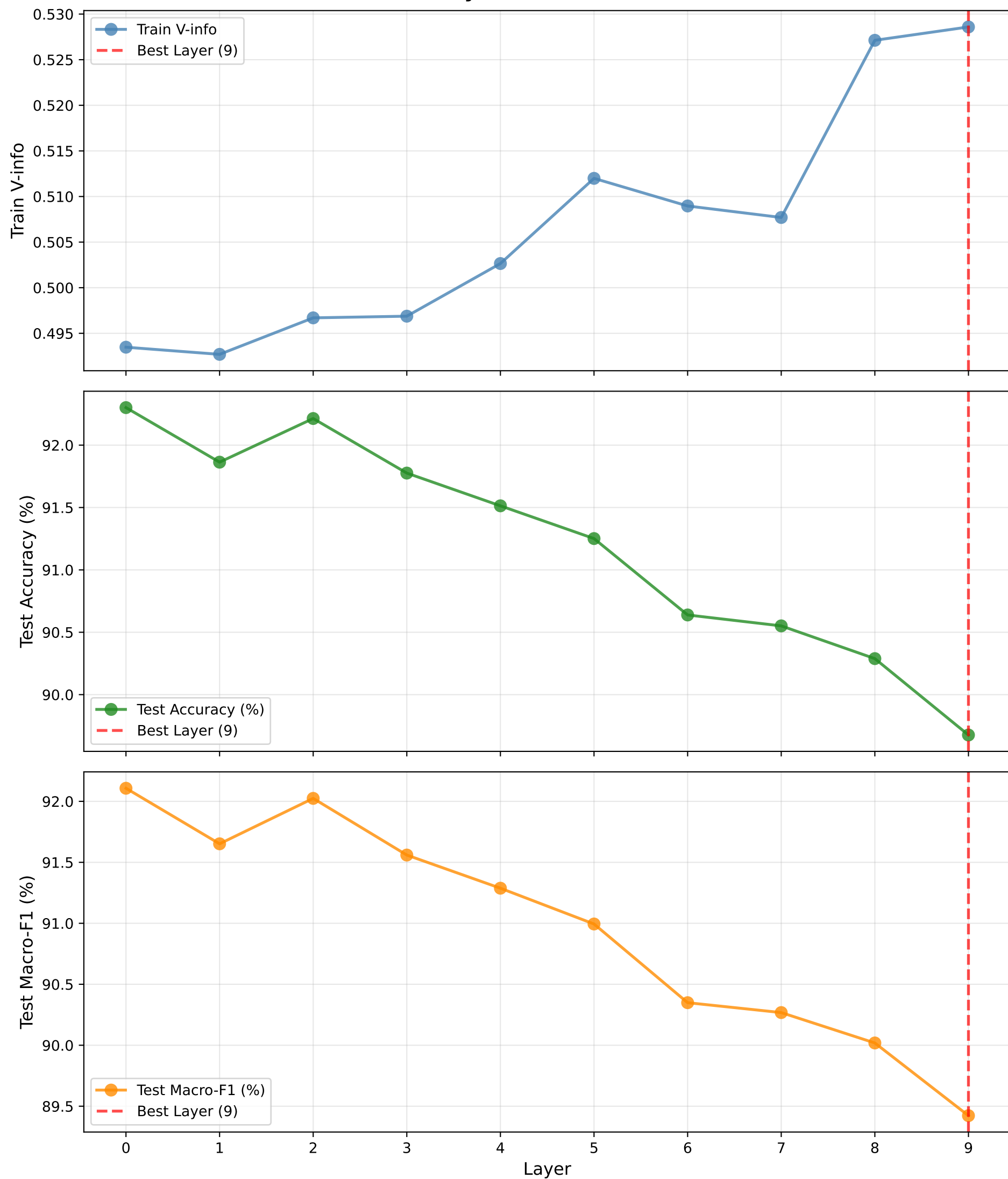
Rice - Layer-wise Metrics
