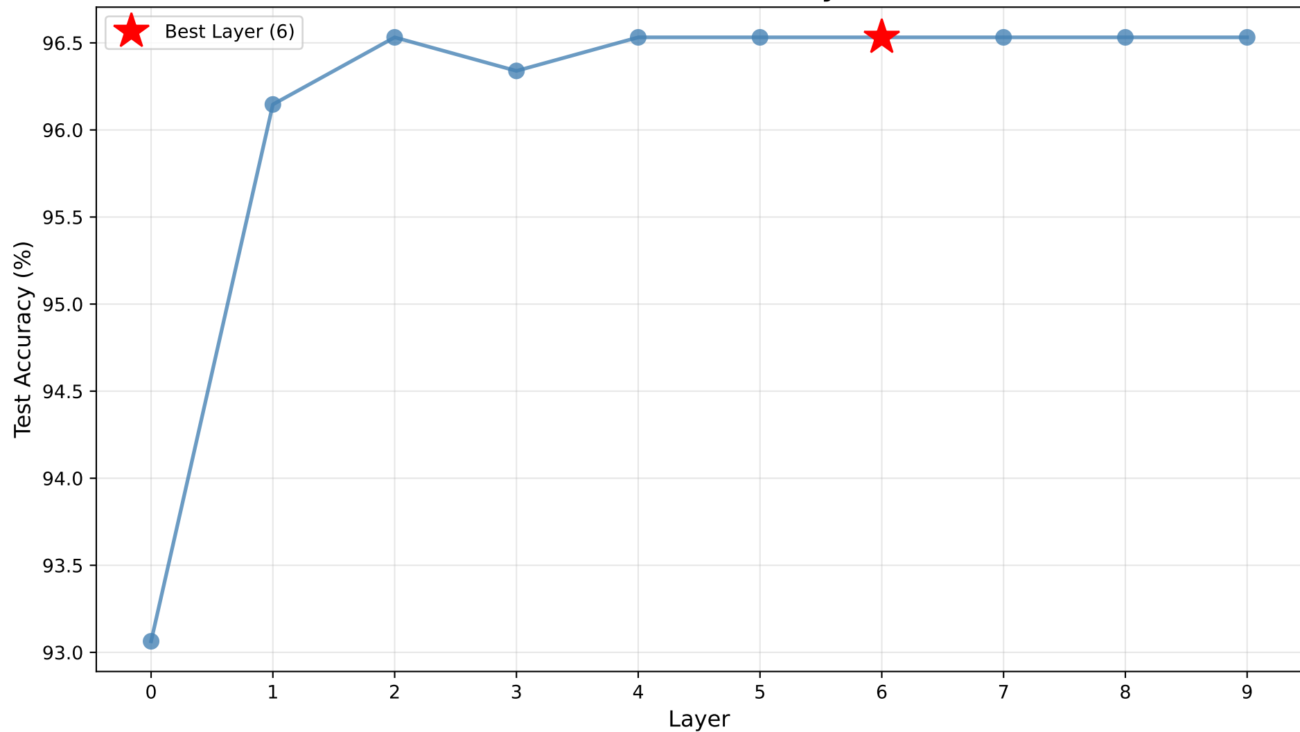
Car - Test Accuracy
