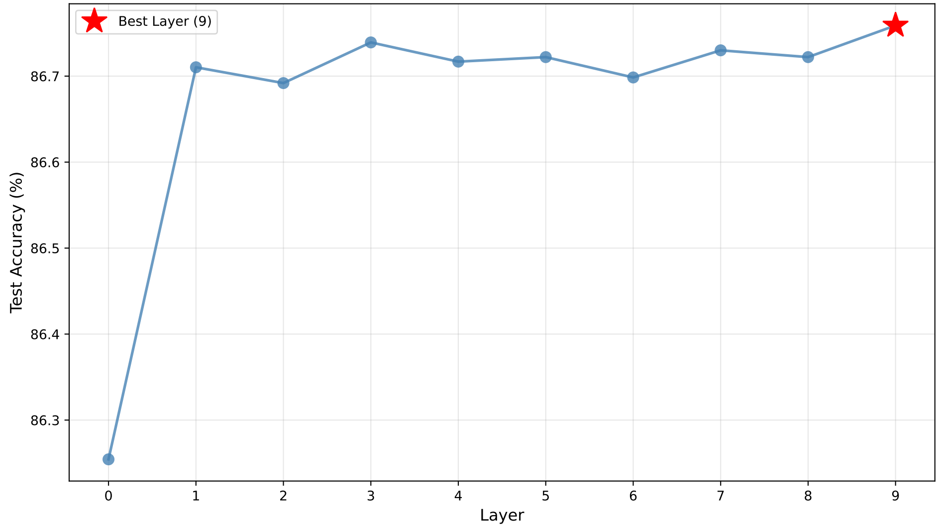
Diabetes - Test Accuracy
