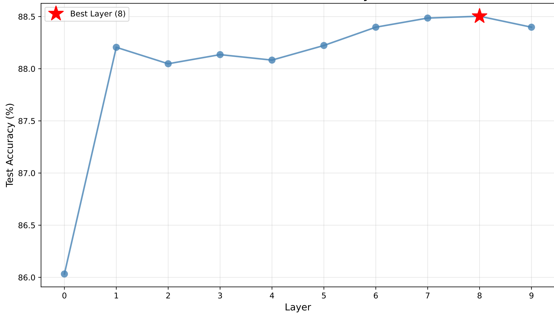
Gamma - Test Accuracy
