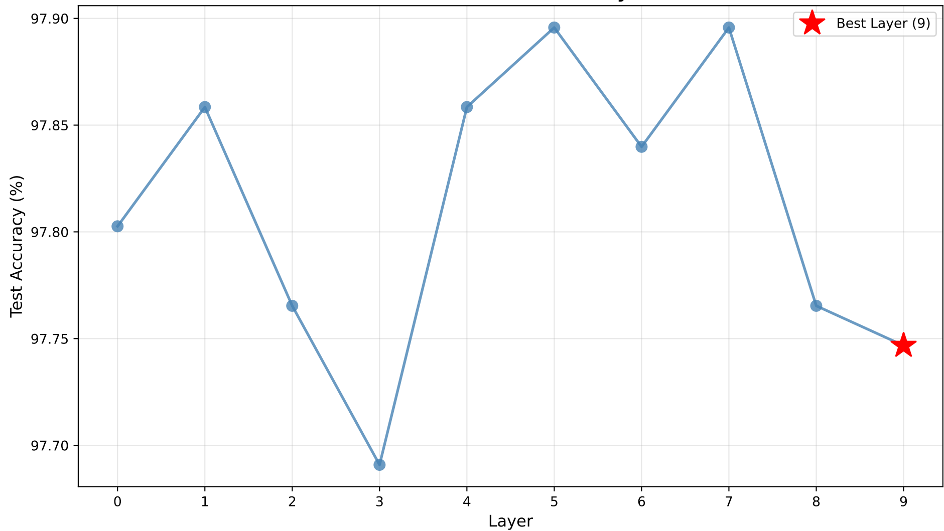
HTRU2 - Test Accuracy
