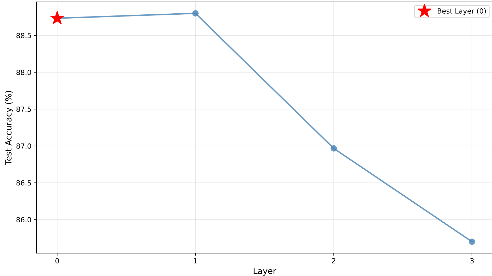
Letter - Test Accuracy
