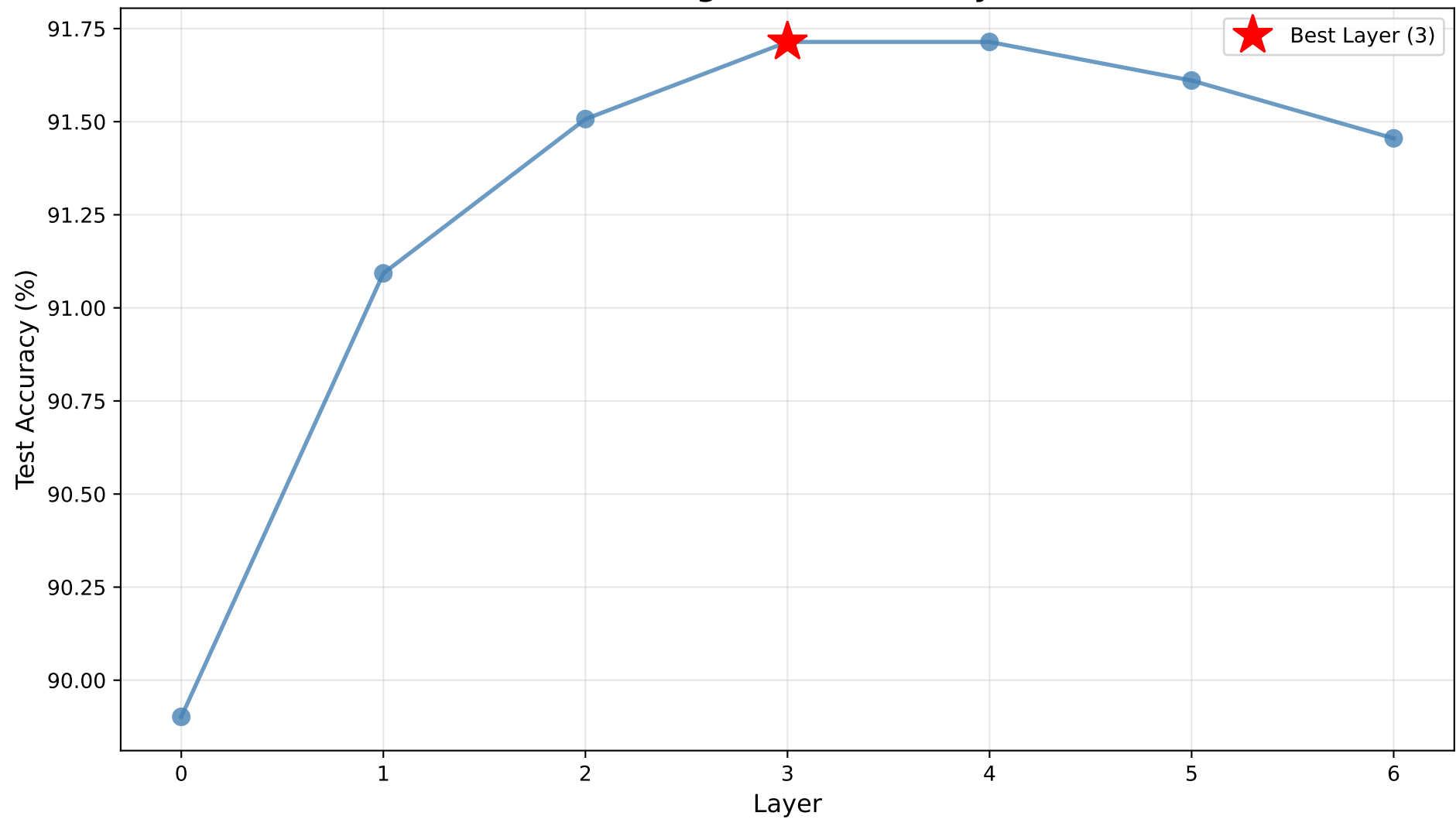
Satimage - Test Accuracy
