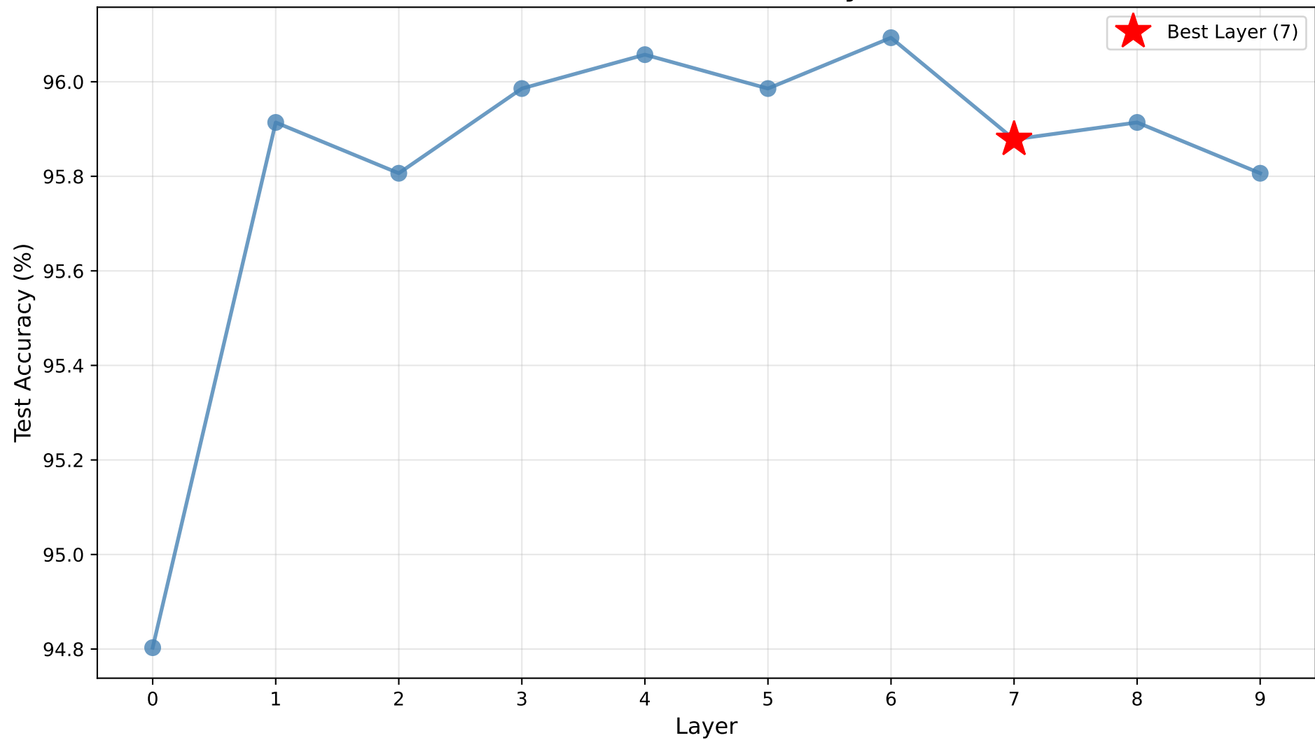
USPS - Test Accuracy
