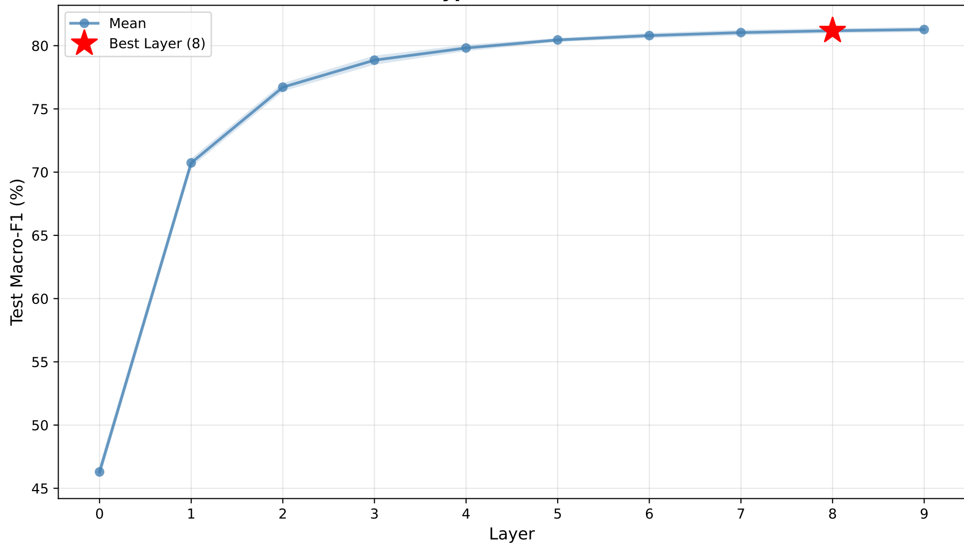
Coverttype - Test Macro-F1
