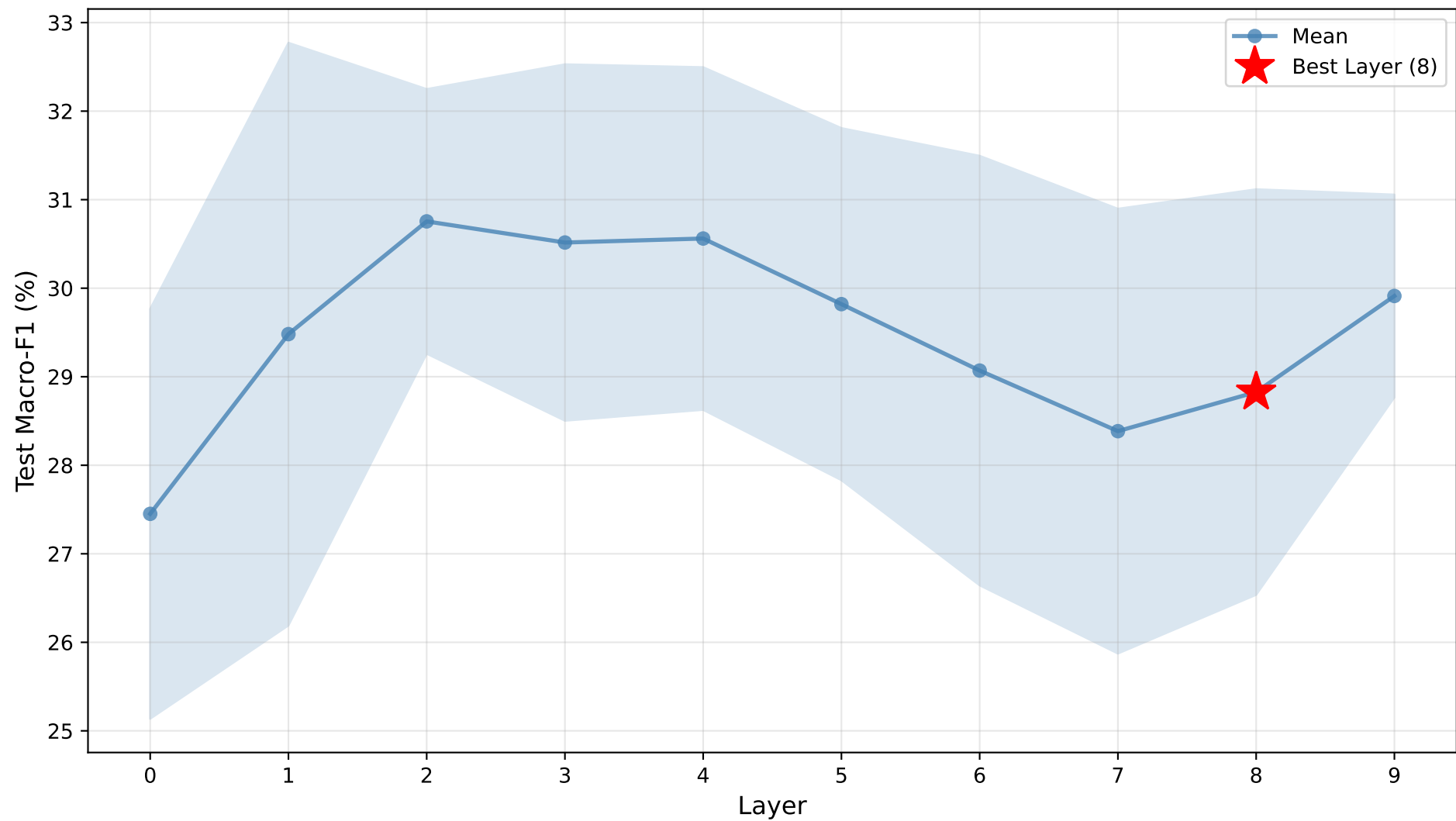
HeartDisease - Test Macro-F1
