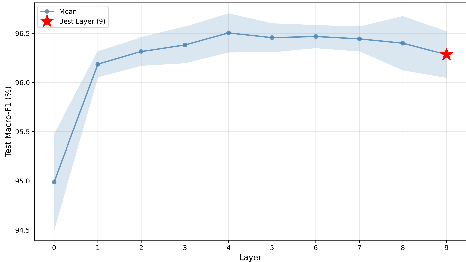
Websites - Test Macro-F1
