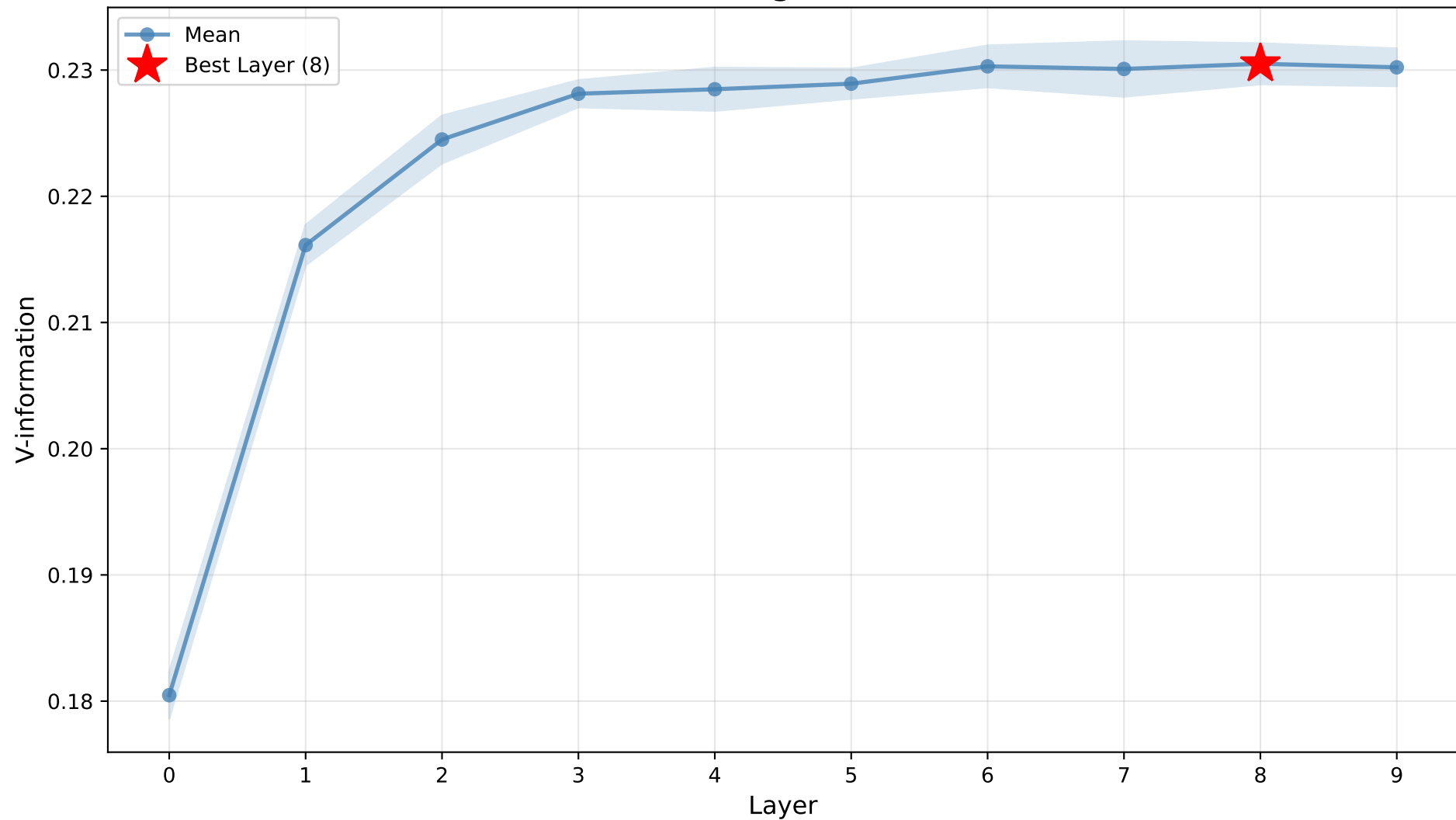
Adult - Training V-information
