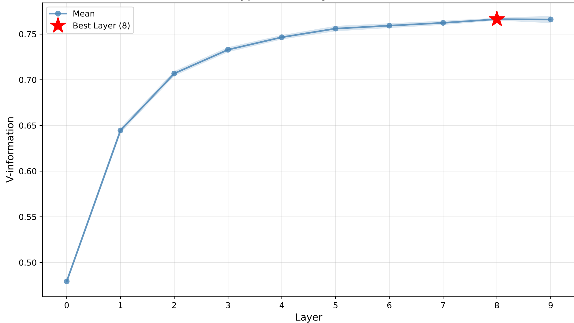
Coverttype - Training V-information
