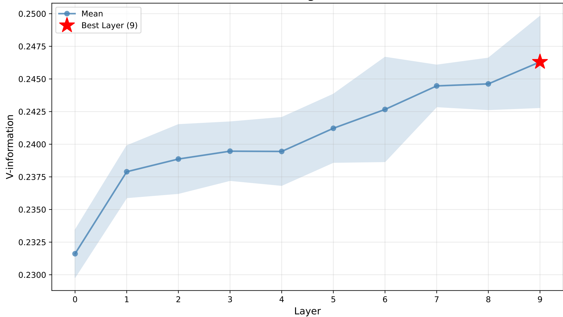
HTRU2 - Training V-information
