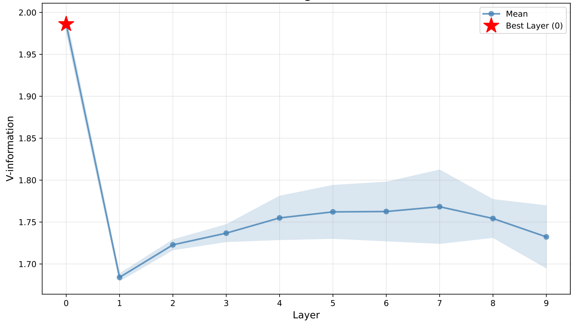
Letter - Training V-information
