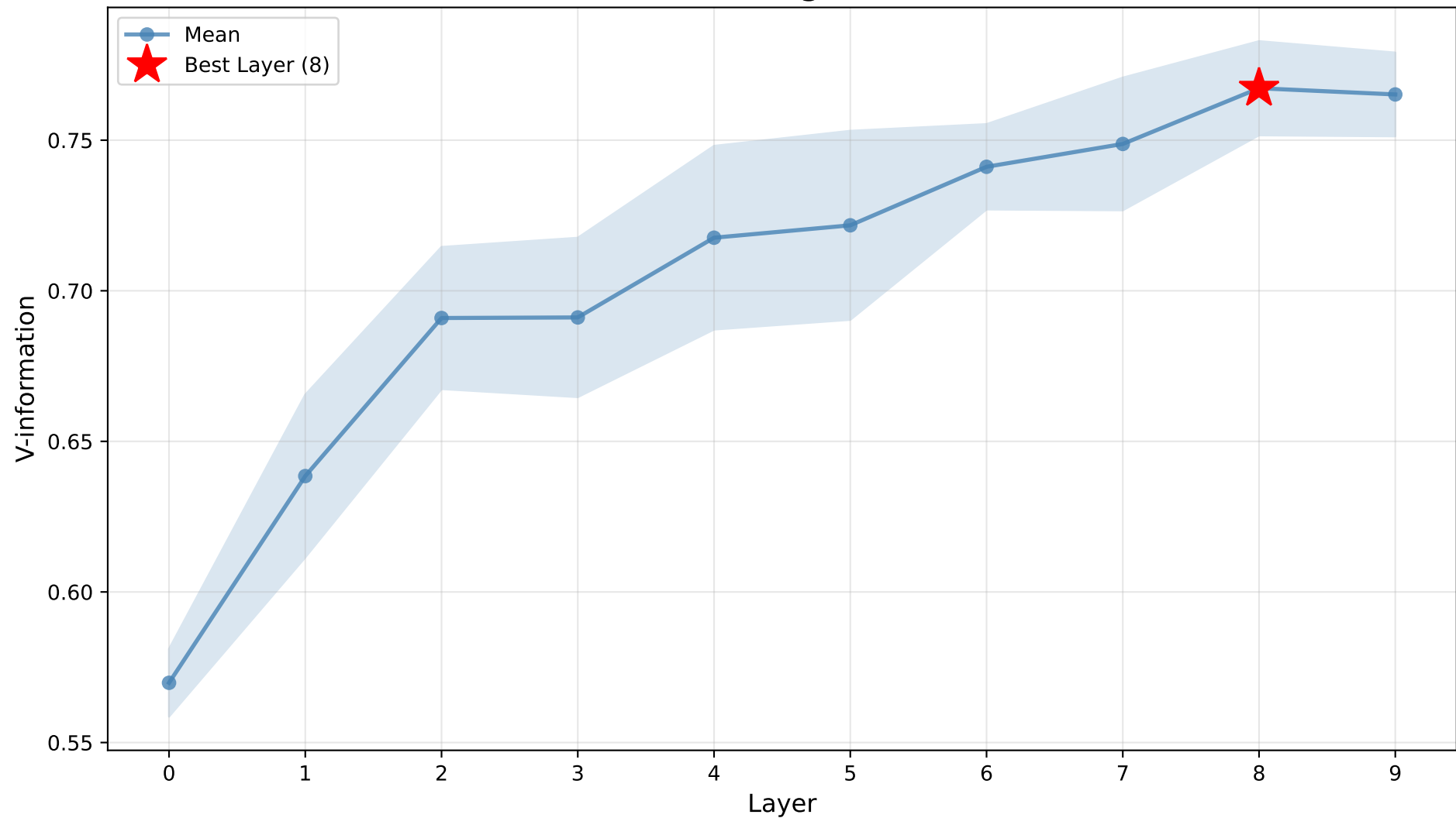
Maternal - Training V-information
