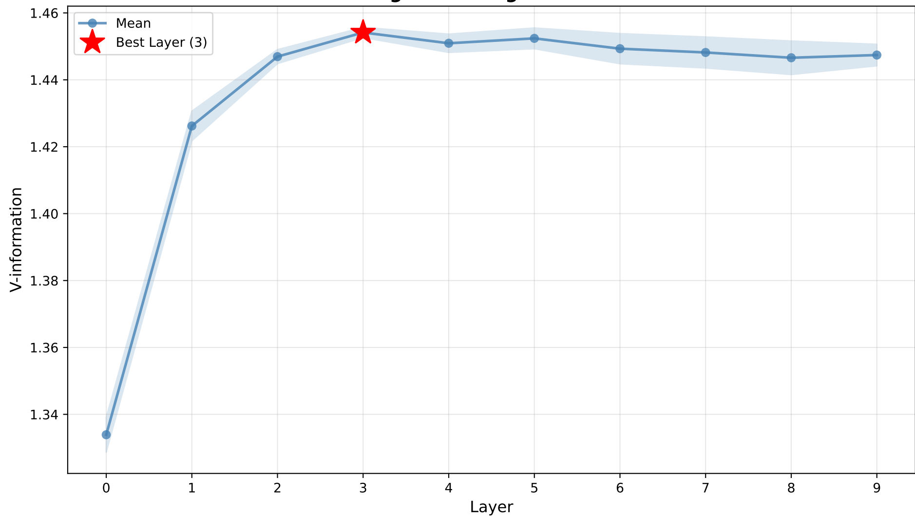
Satimage - Training V-information
