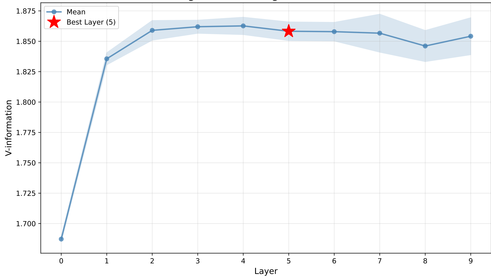
Segment - Training V-information
