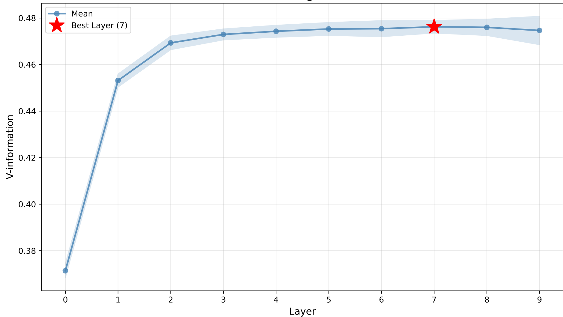
Student - Training V-information
