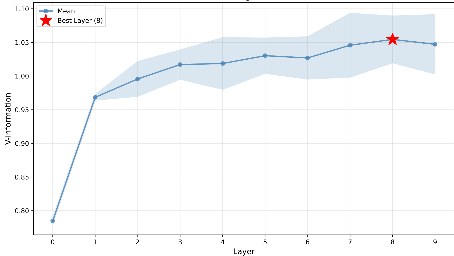
Vehicle - Training V-information
