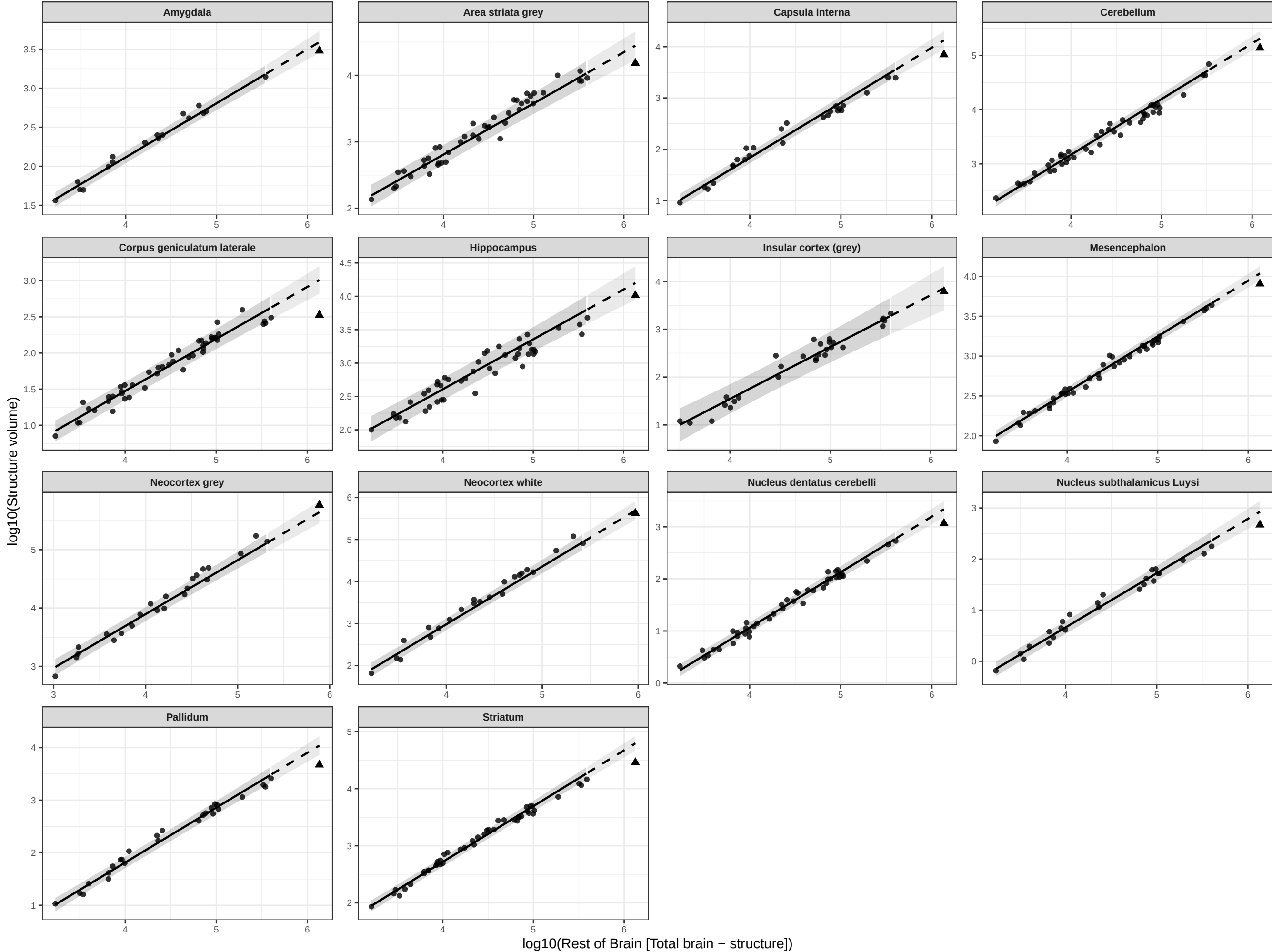
Phylogenetic GLS (BM): All Brain Structures vs Rest of Brain Axes show log10 values. Solid = non-human range; dashed = extrapolation. Human = triangle; fit excludes human.
