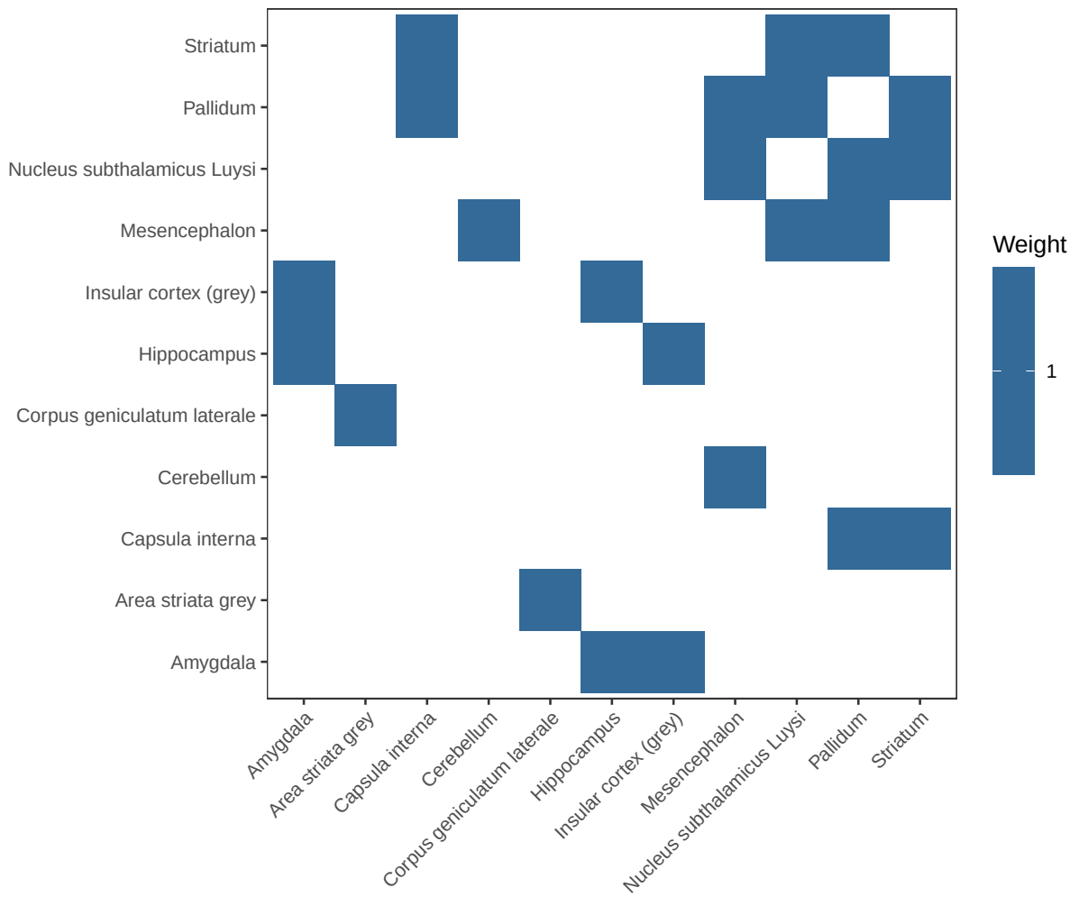
Primary a priori network adjacency matrix
