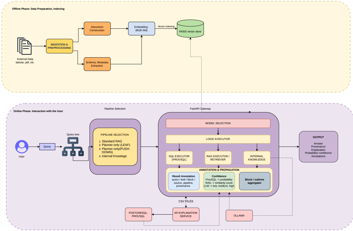
Figure 1: Demo gateway architecture and the main request path.
