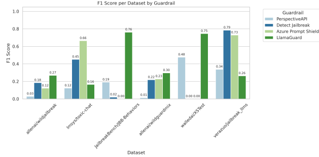
Fig. 5: Comparison of F1 values achieved by the guardrails across all datasets.
