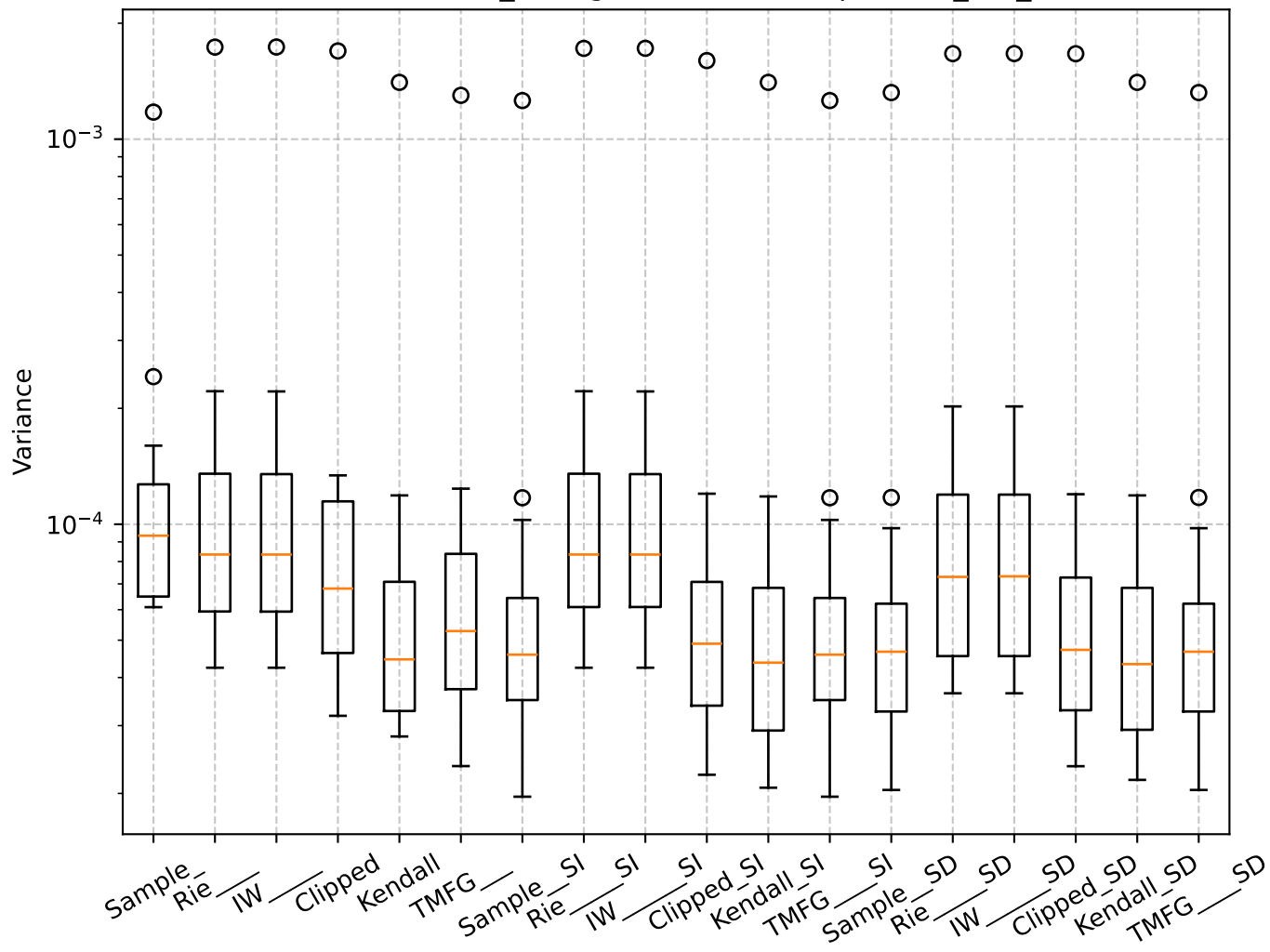
Q=0.53, len_rolling=100: Box Plot per min_var_
