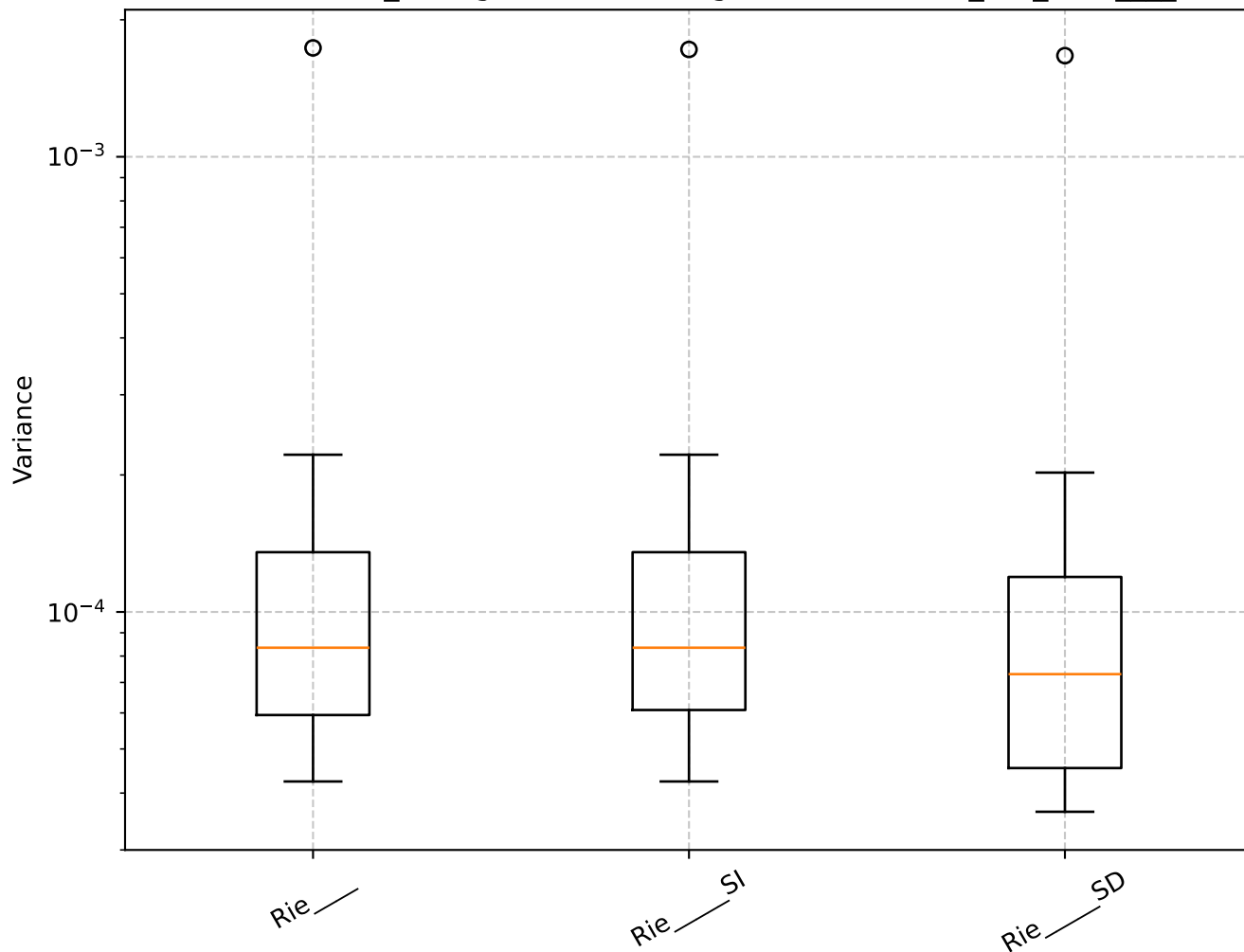
Q=0.54, len_rolling=100: Shrinkage Box Plot - min_var_, Rie____
