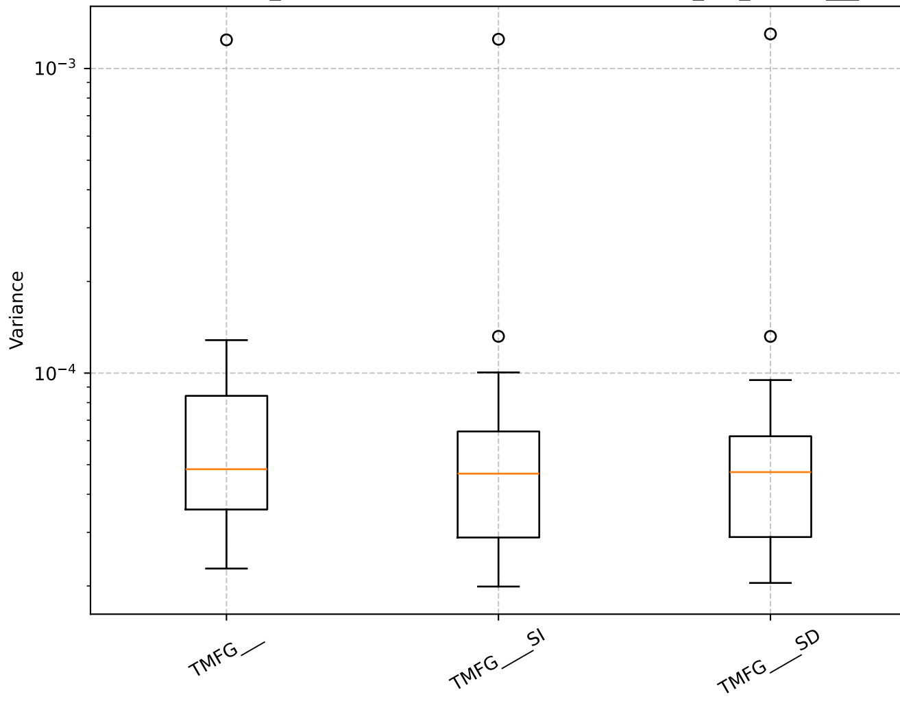
Q=0.56, len_rolling=100: Shrinkage Box Plot - min_var_, TMFG__
