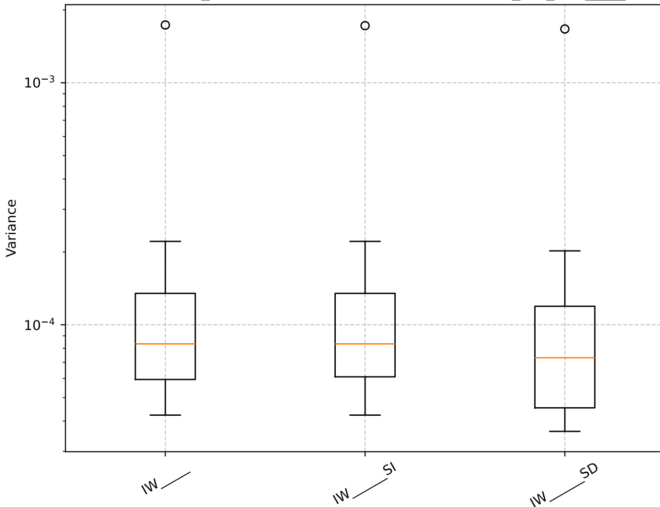
Q=0.57, len_rolling=100: Shrinkage Box Plot - min_var_, IW_____
