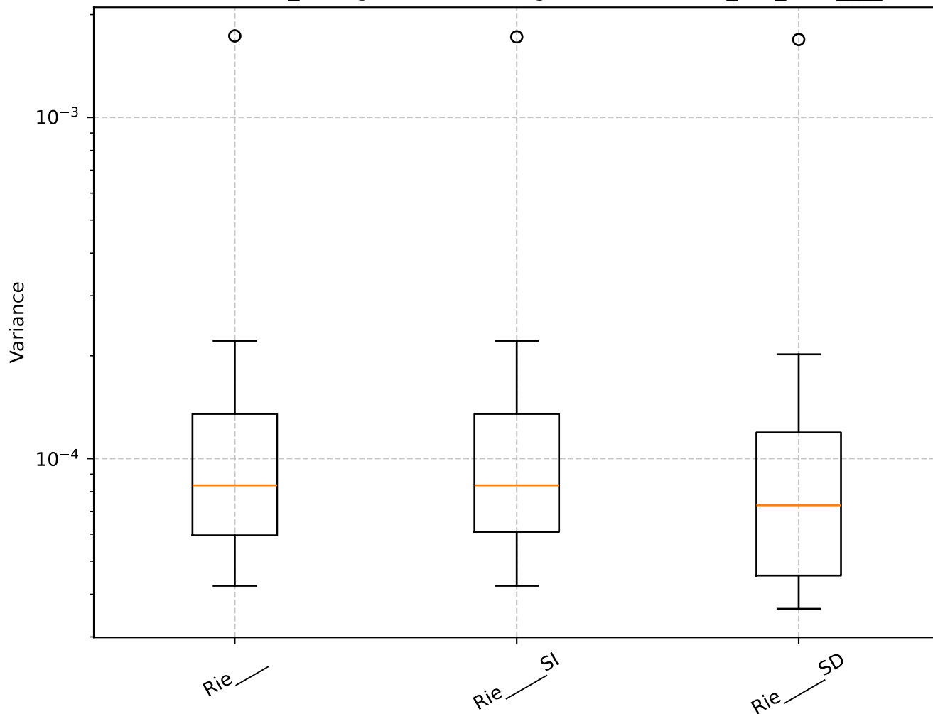
Q=0.57, len_rolling=100: Shrinkage Box Plot - min_var_, Rie____
