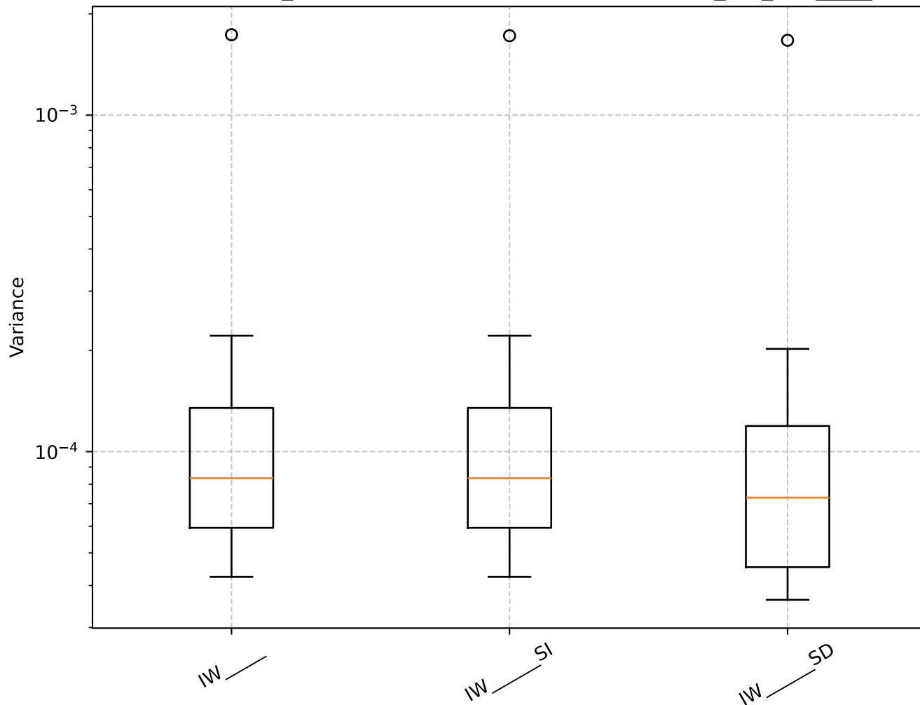
Q=0.58, len_rolling=100: Shrinkage Box Plot - min_var_, IW_____
