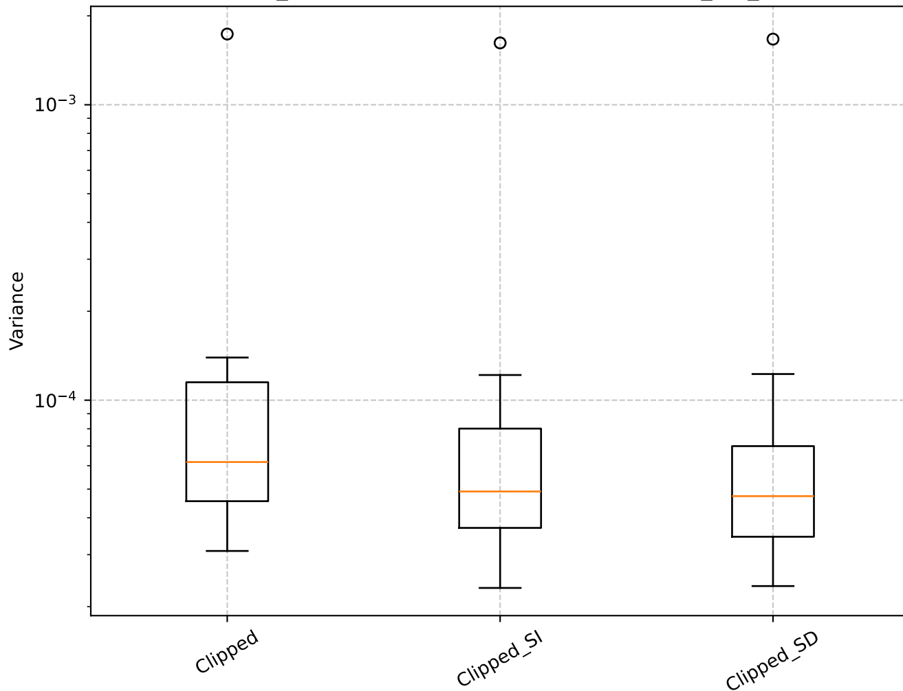
Q=0.59, len_rolling=100: Shrinkage Box Plot - min_var_, Clipped
