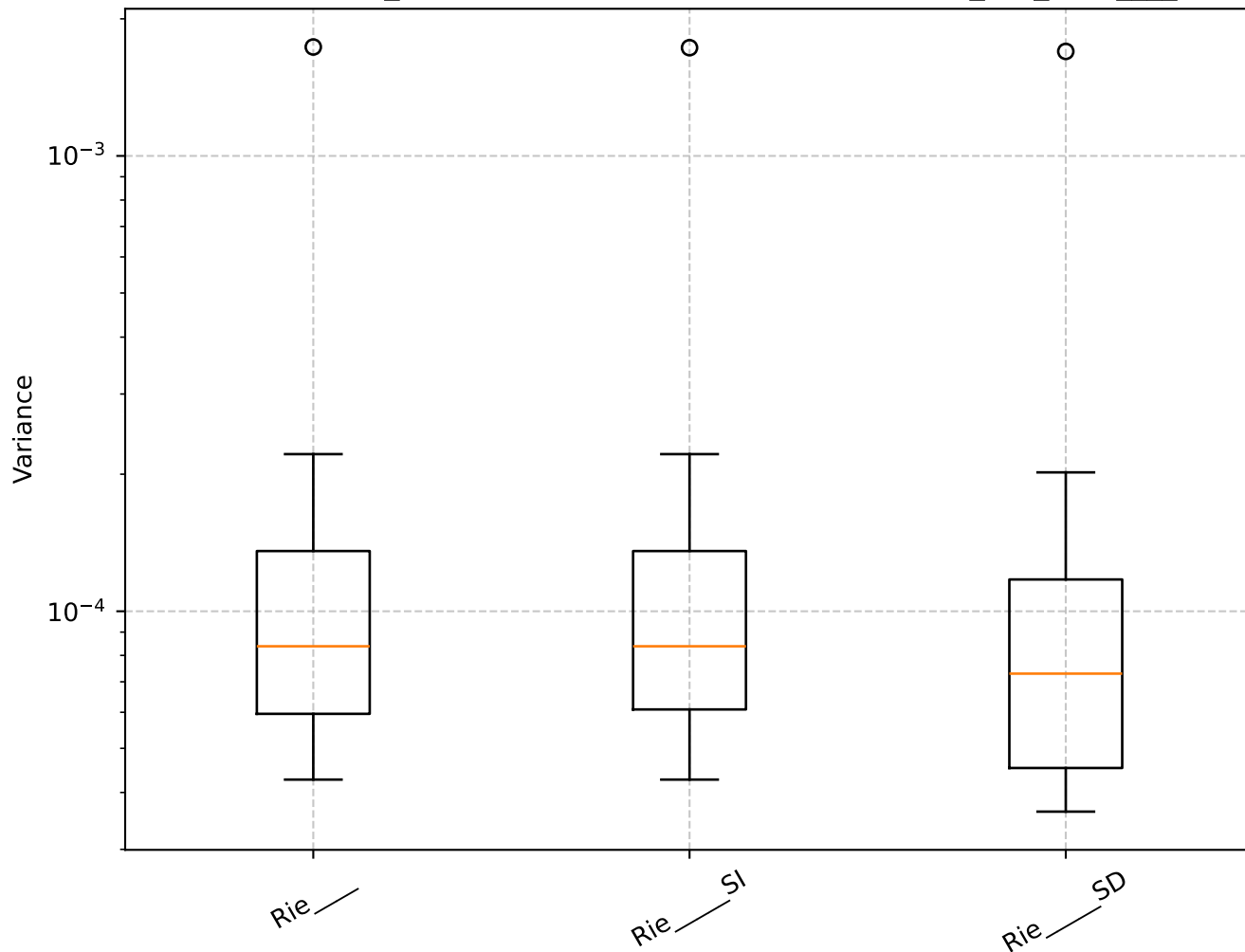
Q=0.63, len_rolling=100: Shrinkage Box Plot - min_var_, Rie____
