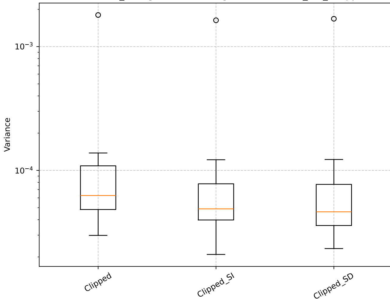
Q=0.65, len_rolling=100: Shrinkage Box Plot - min_var_, Clipped
