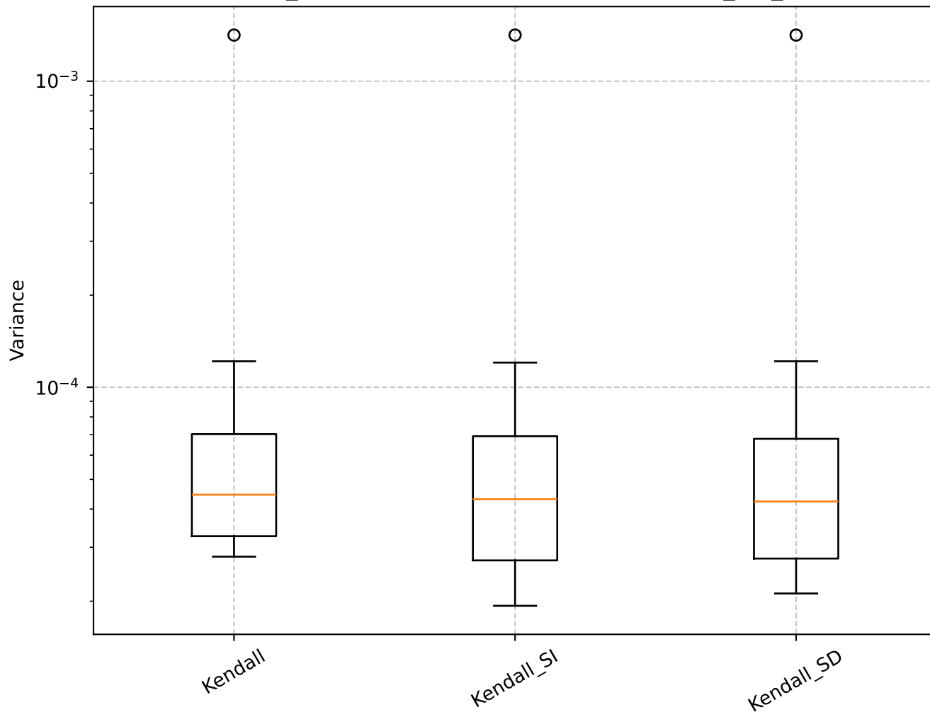
Q=0.66, len_rolling=100: Shrinkage Box Plot - min_var_, Kendall
