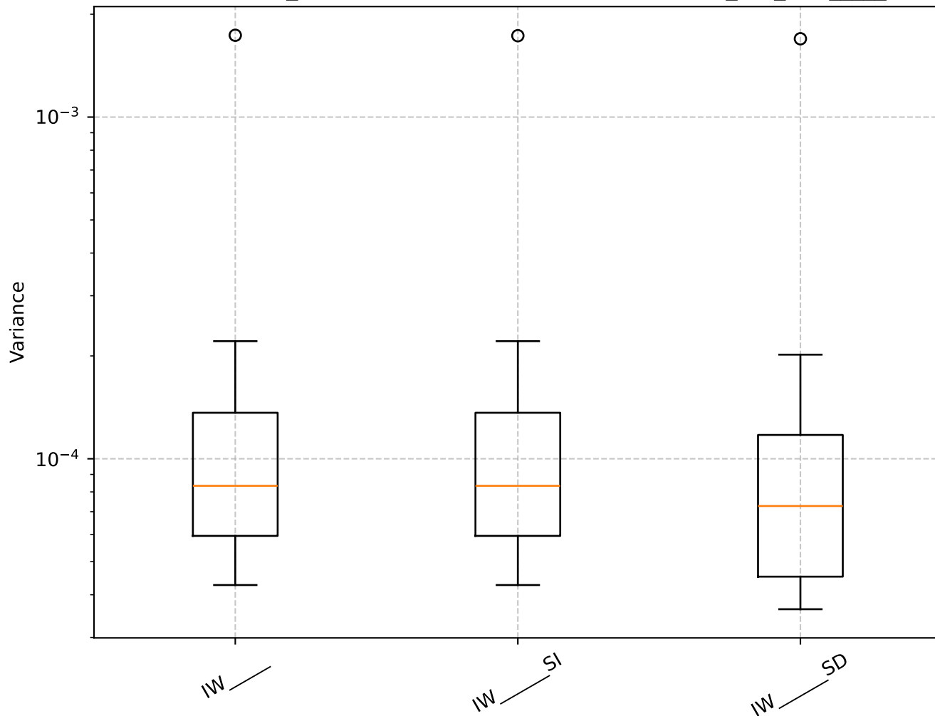
Q=0.67, len_rolling=100: Shrinkage Box Plot - min_var_, IW_____
