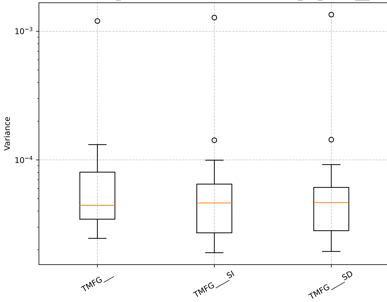
Q=0.68, len_rolling=100: Shrinkage Box Plot - min_var_, TMFG__
